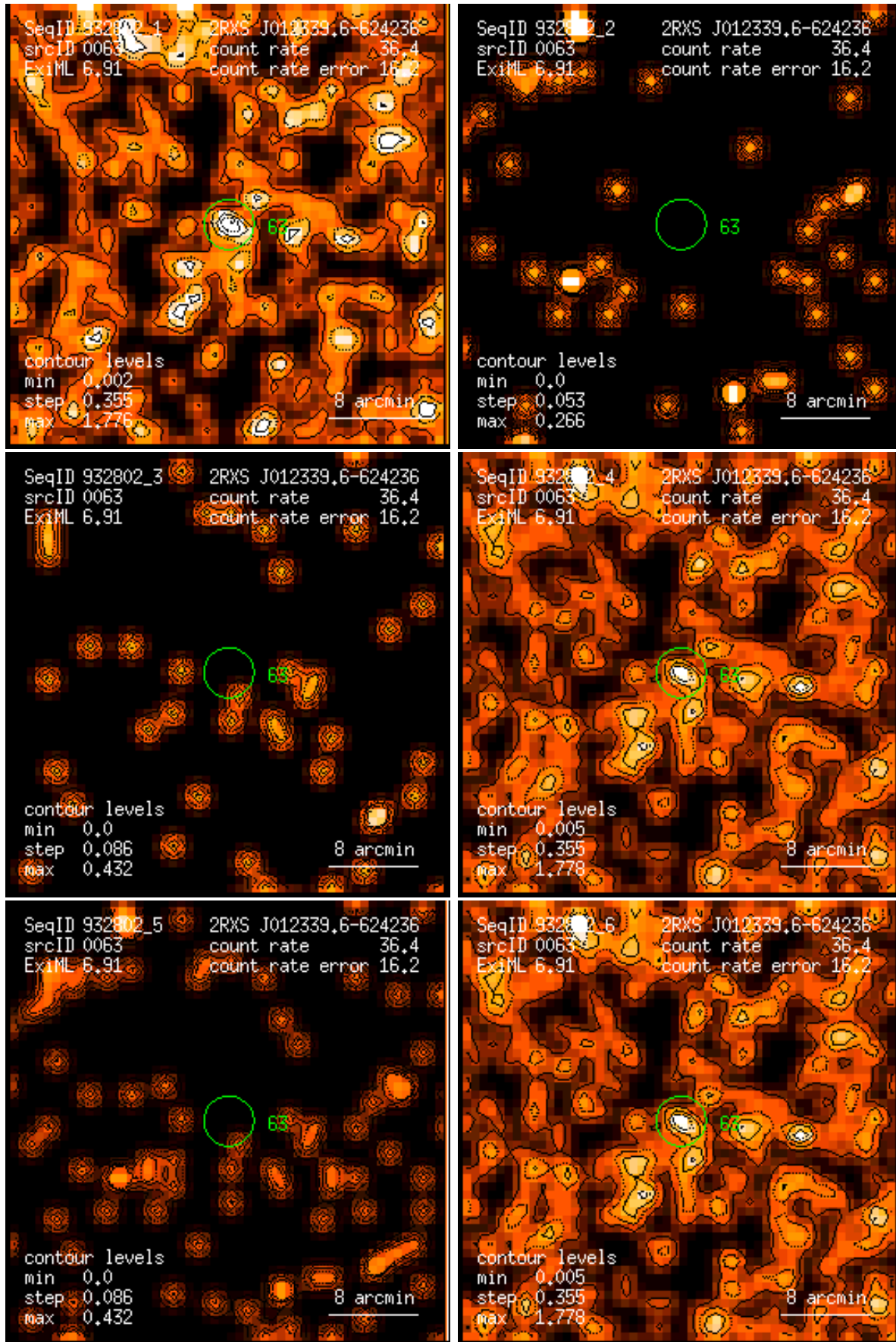
Figure 63: RASS 932802: detection 0063: band rate images, Gaussian filter: (1) PSPC channels 11 – 41, (2) 52 – 90, (3) 91 – 201, (4) 11 – 235, (5) 52 – 201, (6) 11 – 201. Broad band rates in counts/ks. Band rate contour levels in counts/ks/arcmin 2 .
