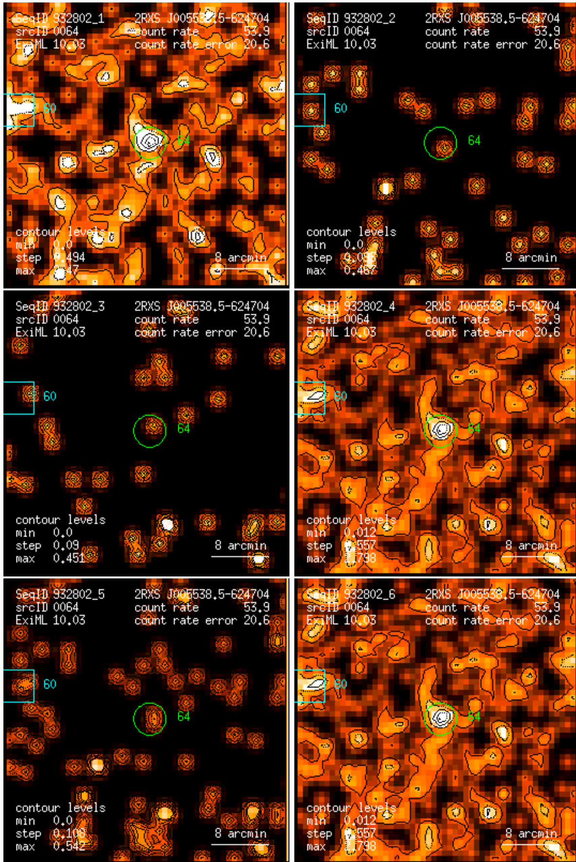
Figure 64: RASS 932802: detection 0064: band rate images, Gaussian filter: (1) PSPC channels 11 – 41, (2) 52 – 90, (3) 91 – 201, (4) 11 – 235, (5) 52 – 201, (6) 11 – 201. Broad band rates in counts/ks. Band rate contour levels in counts/ks/arcmin 2 .
