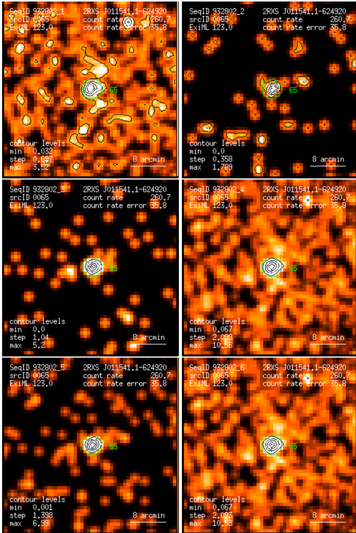
Figure 65: RASS 932802: detection 0065: band rate images, Gaussian filter: (1) PSPC channels 11 – 41, (2) 52 – 90, (3) 91 – 201, (4) 11 – 235, (5) 52 – 201, (6) 11 – 201. Broad band rates in counts/ks. Band rate contour levels in counts/ks/arcmin 2 .
