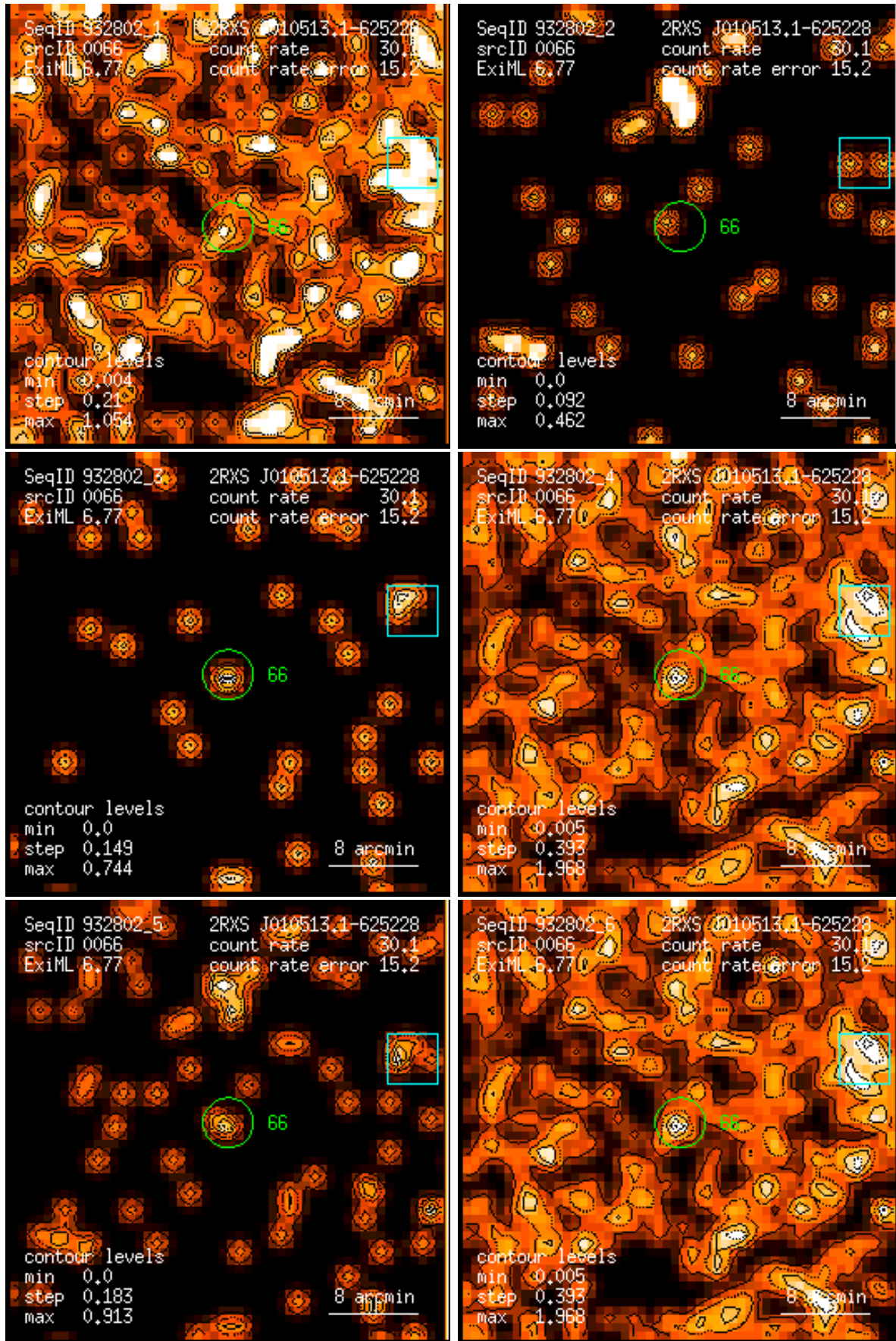
Figure 66: RASS 932802: detection 0066: band rate images, Gaussian filter: (1) PSPC channels 11 – 41, (2) 52 – 90, (3) 91 – 201, (4) 11 – 235, (5) 52 – 201, (6) 11 – 201. Broad band rates in counts/ks. Band rate contour levels in counts/ks/arcmin 2 .
