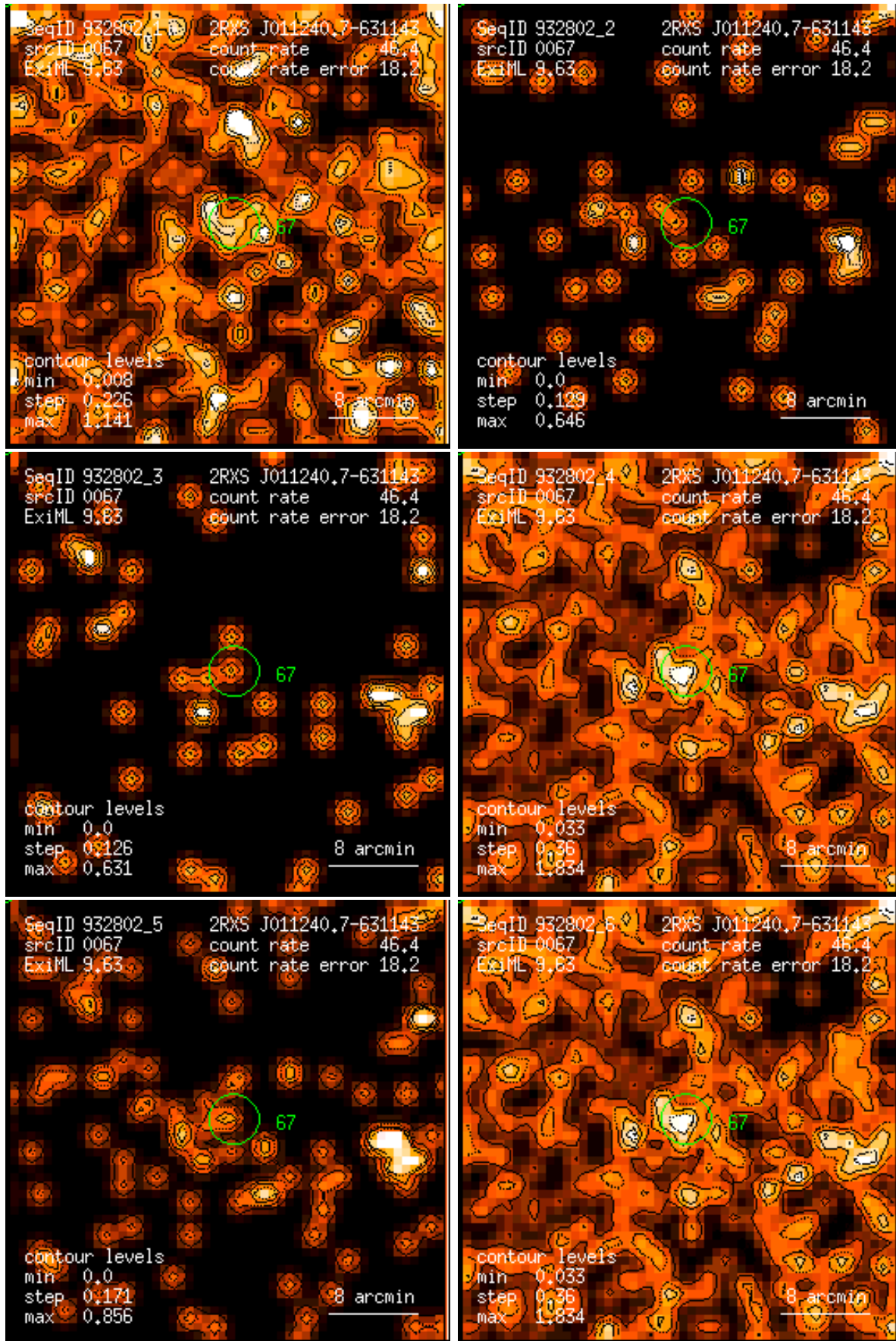
Figure 67: RASS 932802: detection 0067: band rate images, Gaussian filter: (1) PSPC channels 11 – 41, (2) 52 – 90, (3) 91 – 201, (4) 11 – 235, (5) 52 – 201, (6) 11 – 201. Broad band rates in counts/ks. Band rate contour levels in counts/ks/arcmin 2 .
