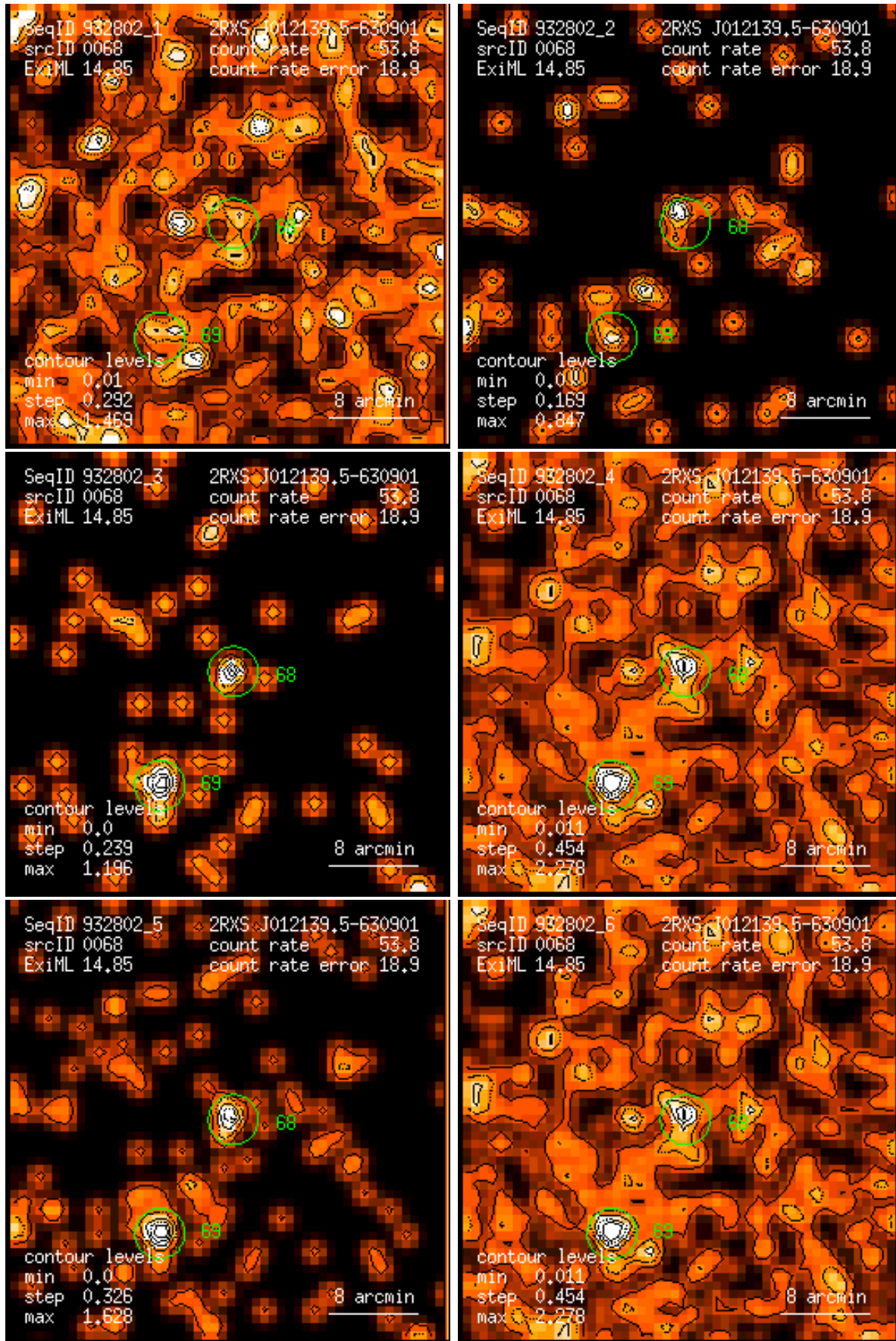
Figure 68: RASS 932802: detection 0068: band rate images, Gaussian filter: (1) PSPC channels 11 – 41, (2) 52 – 90, (3) 91 – 201, (4) 11 – 235, (5) 52 – 201, (6) 11 – 201. Broad band rates in counts/ks. Band rate contour levels in counts/ks/arcmin 2 .
