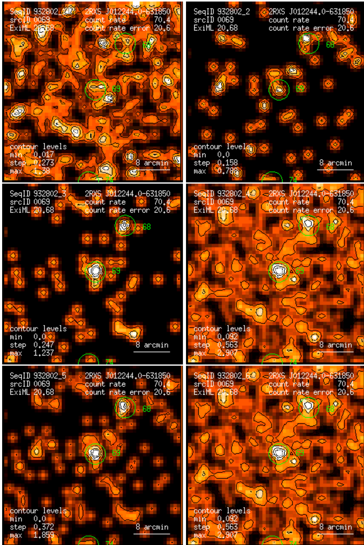
Figure 69: RASS 932802: detection 0069: band rate images, Gaussian filter: (1) PSPC channels 11 – 41, (2) 52 – 90, (3) 91 – 201, (4) 11 – 235, (5) 52 – 201, (6) 11 – 201. Broad band rates in counts/ks. Band rate contour levels in counts/ks/arcmin 2 .
