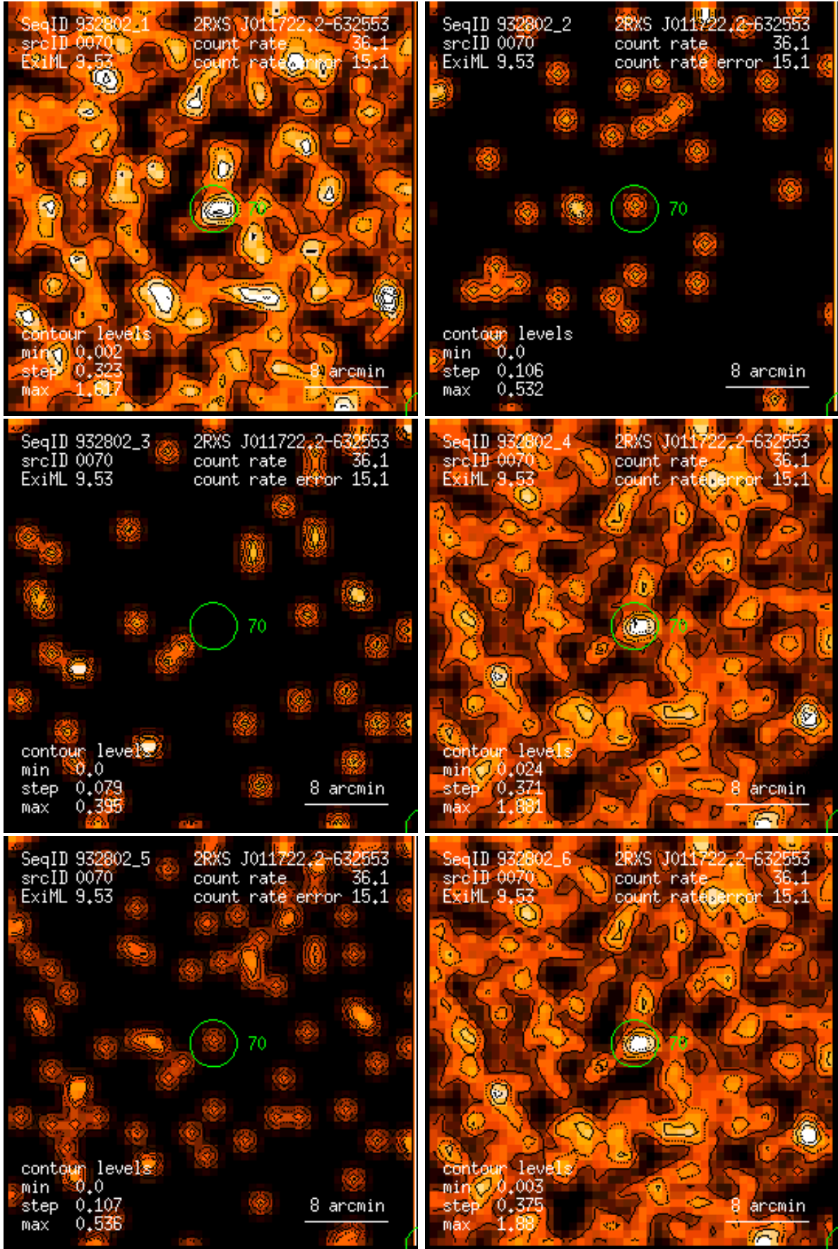
Figure 70: RASS 932802: detection 0070: band rate images, Gaussian filter: (1) PSPC channels 11 – 41, (2) 52 – 90, (3) 91 – 201, (4) 11 – 235, (5) 52 – 201, (6) 11 – 201. Broad band rates in counts/ks. Band rate contour levels in counts/ks/arcmin 2 .
