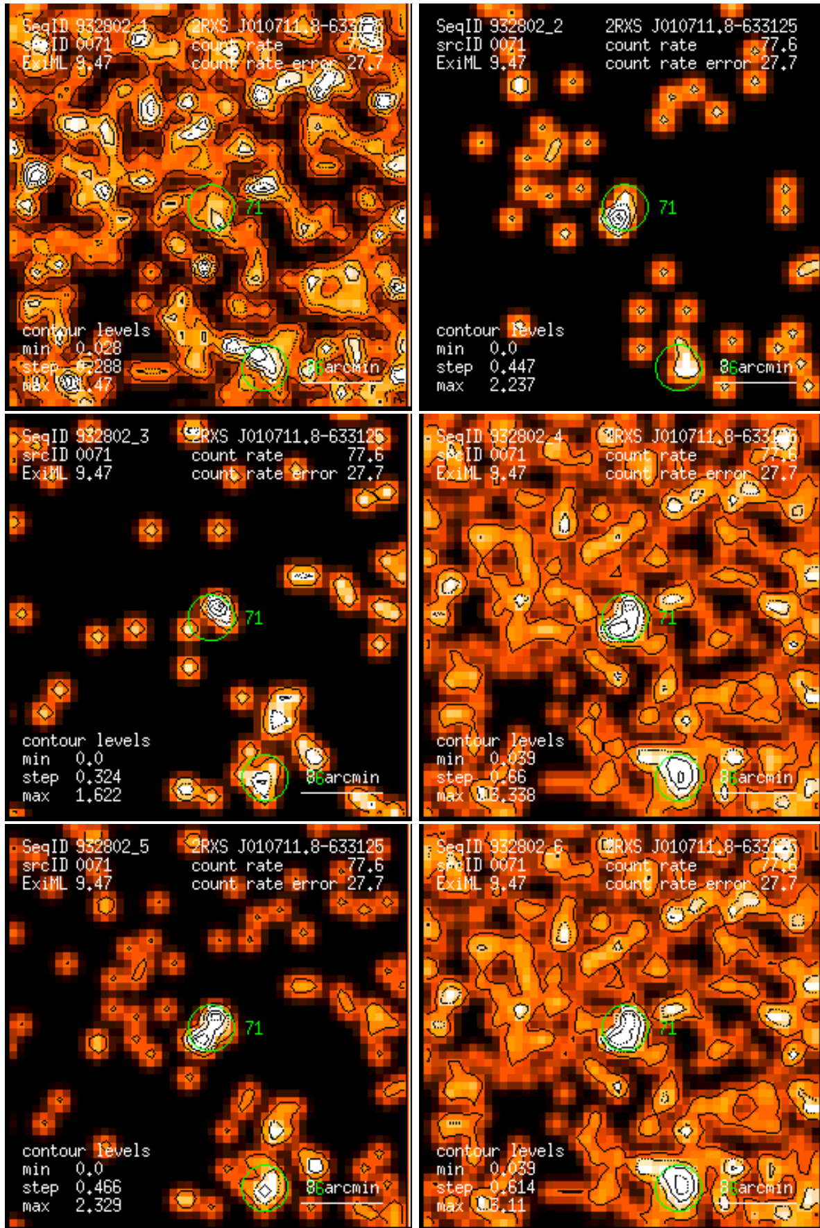
Figure 71: RASS 932802: detection 0071: band rate images, Gaussian filter: (1) PSPC channels 11 – 41, (2) 52 – 90, (3) 91 – 201, (4) 11 – 235, (5) 52 – 201, (6) 11 – 201. Broad band rates in counts/ks. Band rate contour levels in counts/ks/arcmin 2 .
