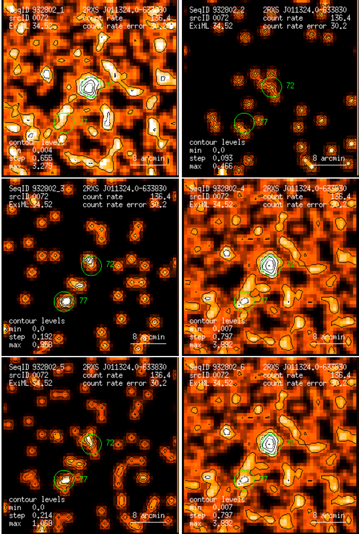
Figure 72: RASS 932802: detection 0072: band rate images, Gaussian filter: (1) PSPC channels 11 – 41, (2) 52 – 90, (3) 91 – 201, (4) 11 – 235, (5) 52 – 201, (6) 11 – 201. Broad band rates in counts/ks. Band rate contour levels in counts/ks/arcmin 2 .
