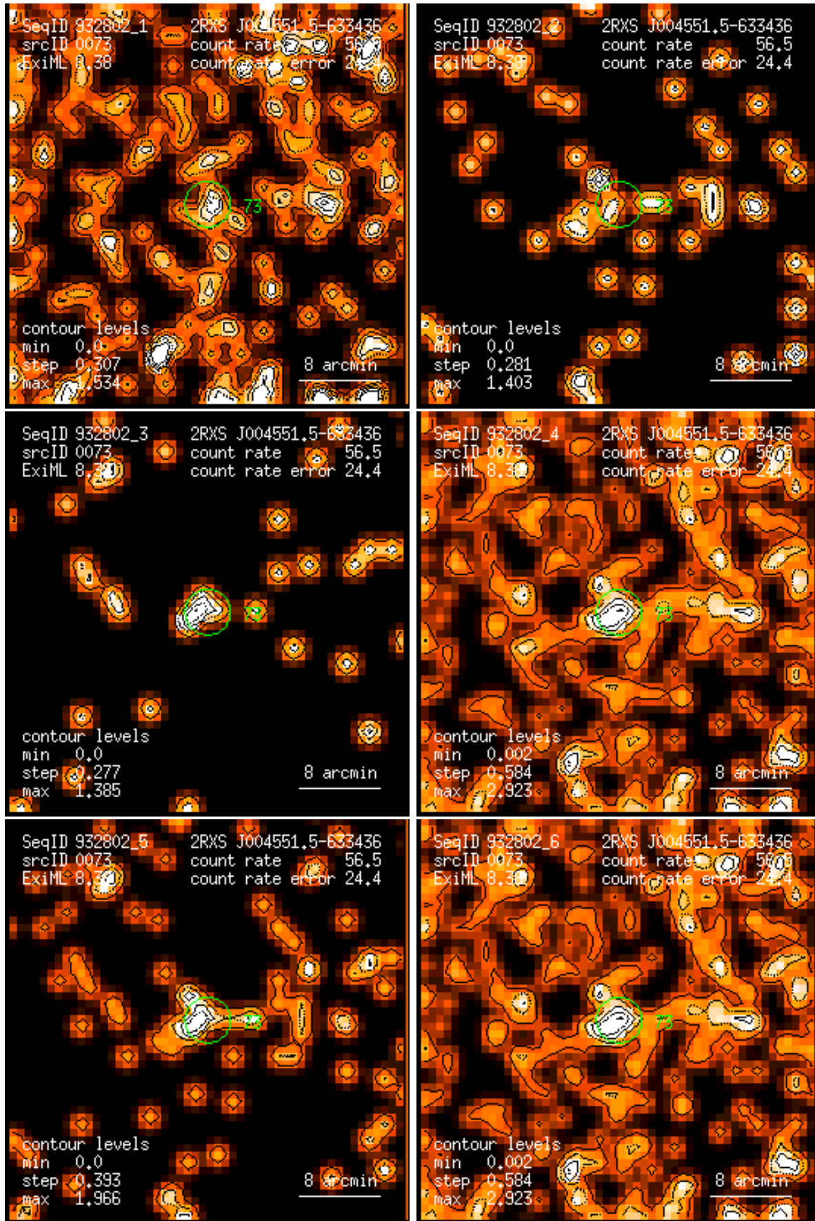
Figure 73: RASS 932802: detection 0073: band rate images, Gaussian filter: (1) PSPC channels 11 – 41, (2) 52 – 90, (3) 91 – 201, (4) 11 – 235, (5) 52 – 201, (6) 11 – 201. Broad band rates in counts/ks. Band rate contour levels in counts/ks/arcmin 2 .
