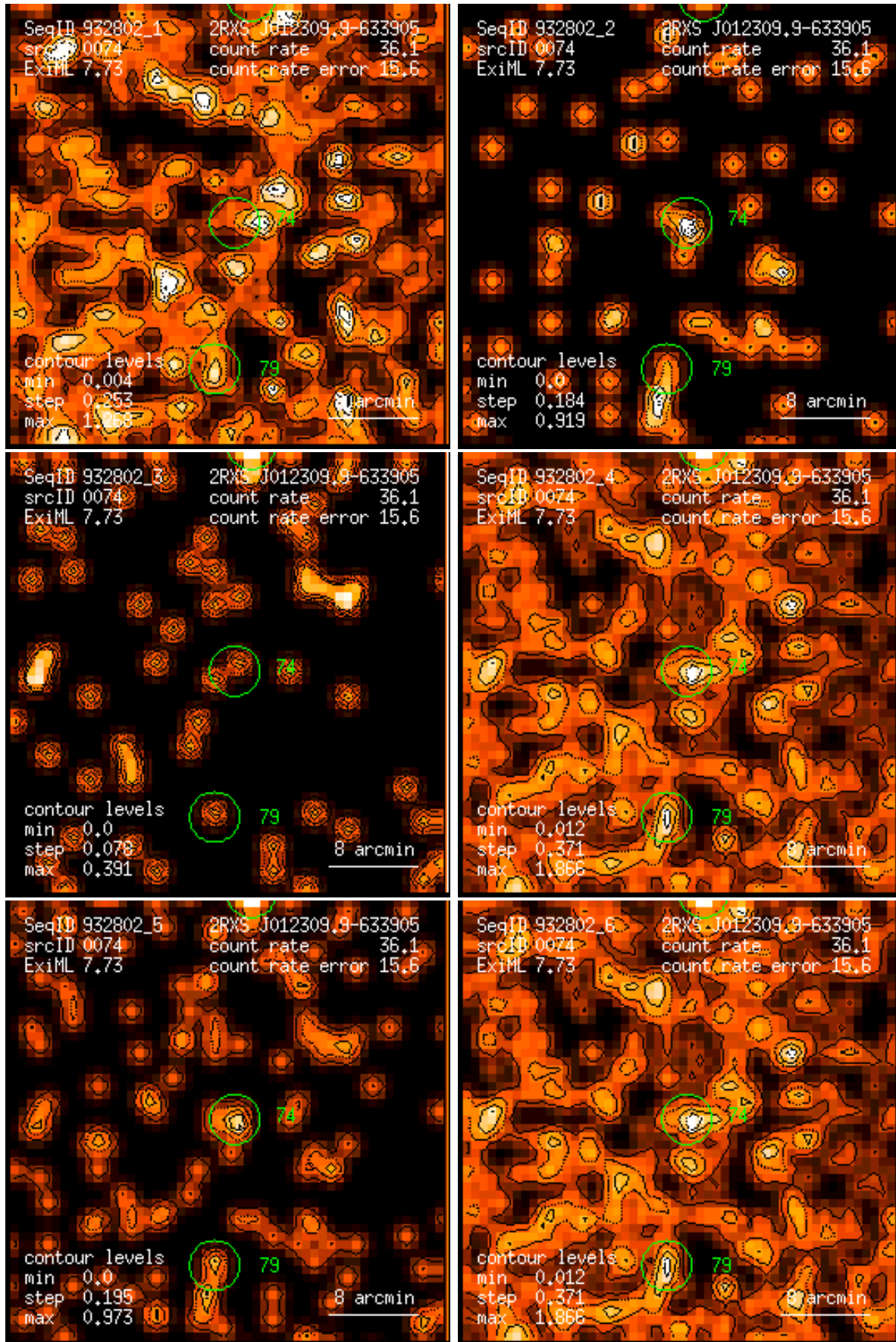
Figure 74: RASS 932802: detection 0074: band rate images, Gaussian filter: (1) PSPC channels 11 – 41, (2) 52 – 90, (3) 91 – 201, (4) 11 – 235, (5) 52 – 201, (6) 11 – 201. Broad band rates in counts/ks. Band rate contour levels in counts/ks/arcmin 2 .
