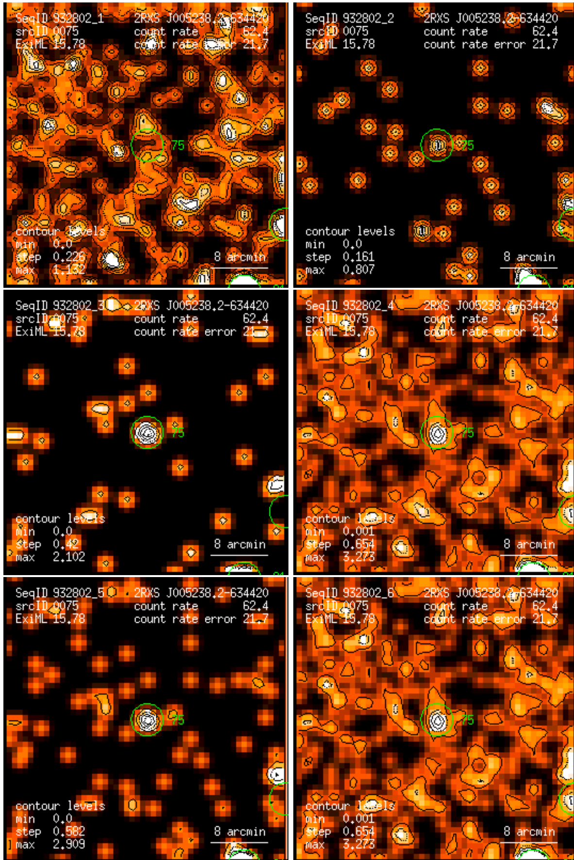
Figure 75: RASS 932802: detection 0075: band rate images, Gaussian filter: (1) PSPC channels 11 – 41, (2) 52 – 90, (3) 91 – 201, (4) 11 – 235, (5) 52 – 201, (6) 11 – 201. Broad band rates in counts/ks. Band rate contour levels in counts/ks/arcmin 2 .
