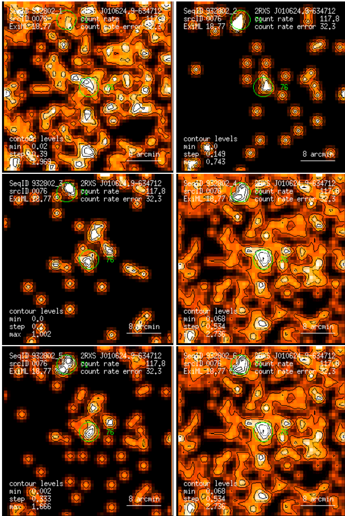
Figure 76: RASS 932802: detection 0076: band rate images, Gaussian filter: (1) PSPC channels 11 – 41, (2) 52 – 90, (3) 91 – 201, (4) 11 – 235, (5) 52 – 201, (6) 11 – 201. Broad band rates in counts/ks. Band rate contour levels in counts/ks/arcmin 2 .
