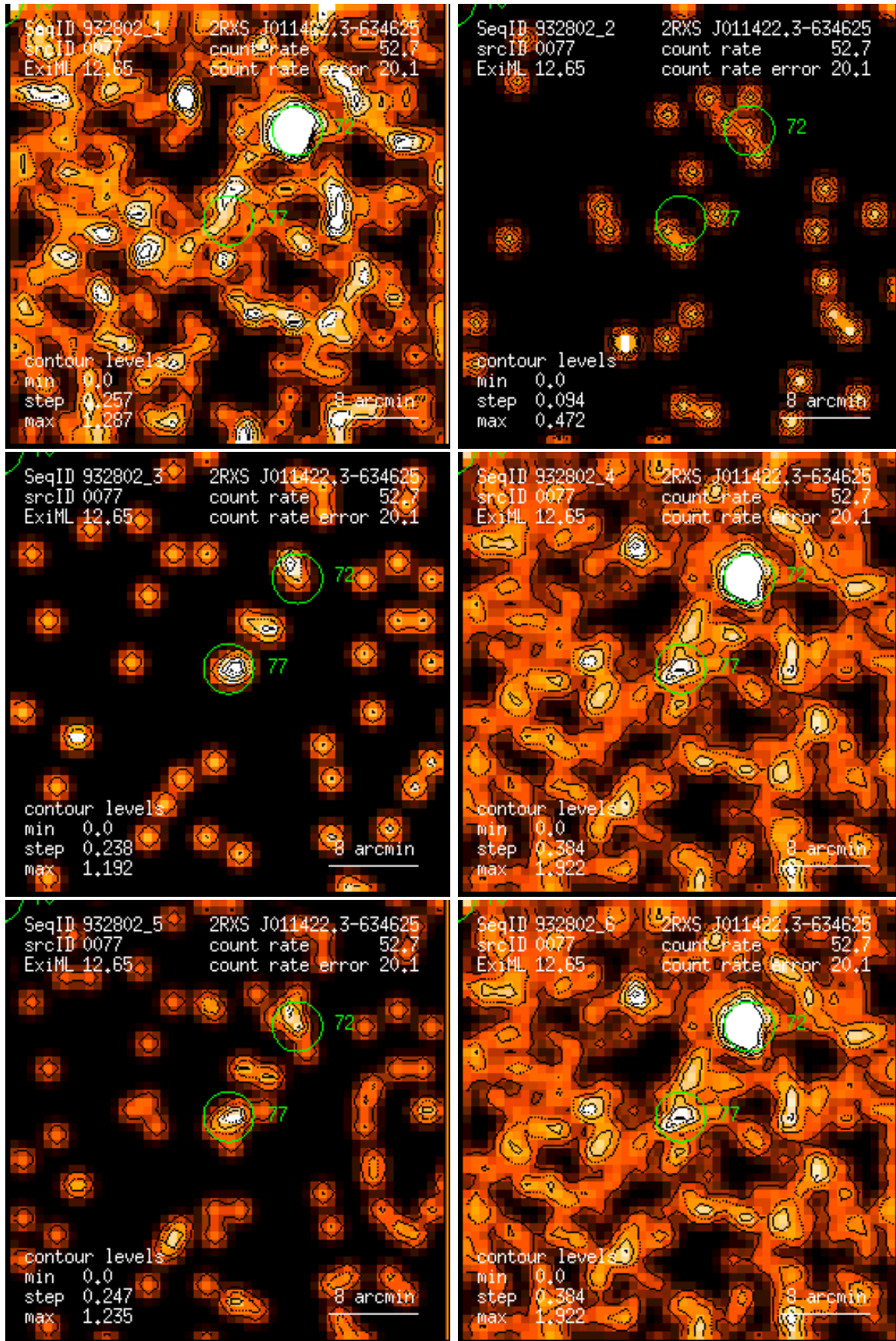
Figure 77: RASS 932802: detection 0077: band rate images, Gaussian filter: (1) PSPC channels 11 – 41, (2) 52 – 90, (3) 91 – 201, (4) 11 – 235, (5) 52 – 201, (6) 11 – 201. Broad band rates in counts/ks. Band rate contour levels in counts/ks/arcmin 2 .
