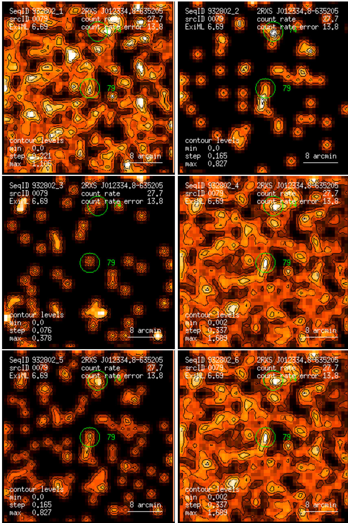
Figure 79: RASS 932802: detection 0079: band rate images, Gaussian filter: (1) PSPC channels 11 – 41, (2) 52 – 90, (3) 91 – 201, (4) 11 – 235, (5) 52 – 201, (6) 11 – 201. Broad band rates in counts/ks. Band rate contour levels in counts/ks/arcmin 2 .
