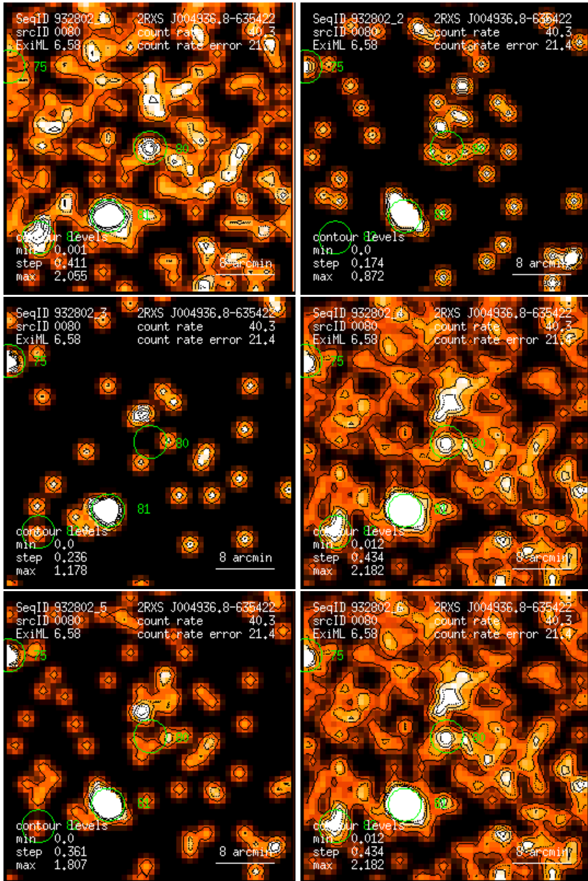
Figure 80: RASS 932802: detection 0080: band rate images, Gaussian filter: (1) PSPC channels 11 – 41, (2) 52 – 90, (3) 91 – 201, (4) 11 – 235, (5) 52 – 201, (6) 11 – 201. Broad band rates in counts/ks. Band rate contour levels in counts/ks/arcmin 2 .
