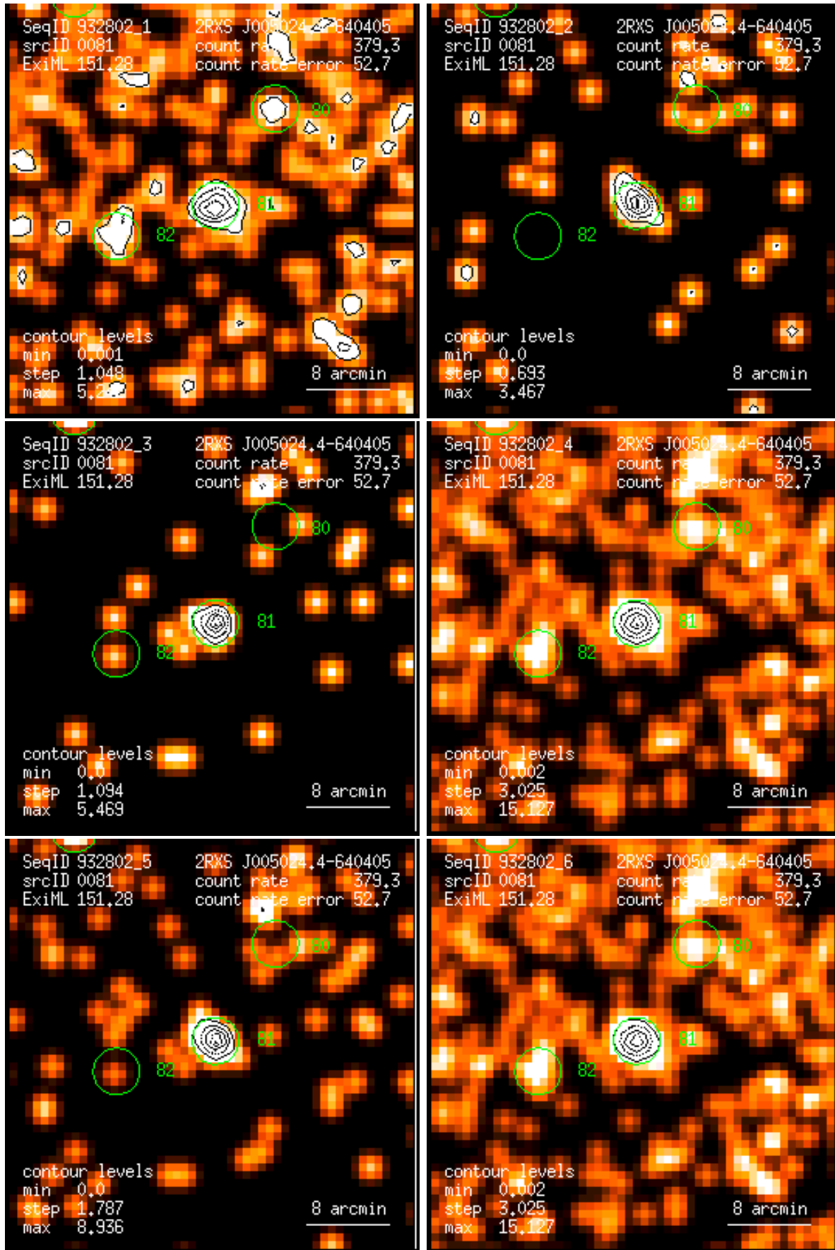
Figure 81: RASS 932802: detection 0081: band rate images, Gaussian filter: (1) PSPC channels 11 – 41, (2) 52 – 90, (3) 91 – 201, (4) 11 – 235, (5) 52 – 201, (6) 11 – 201. Broad band rates in counts/ks. Band rate contour levels in counts/ks/arcmin 2 .
