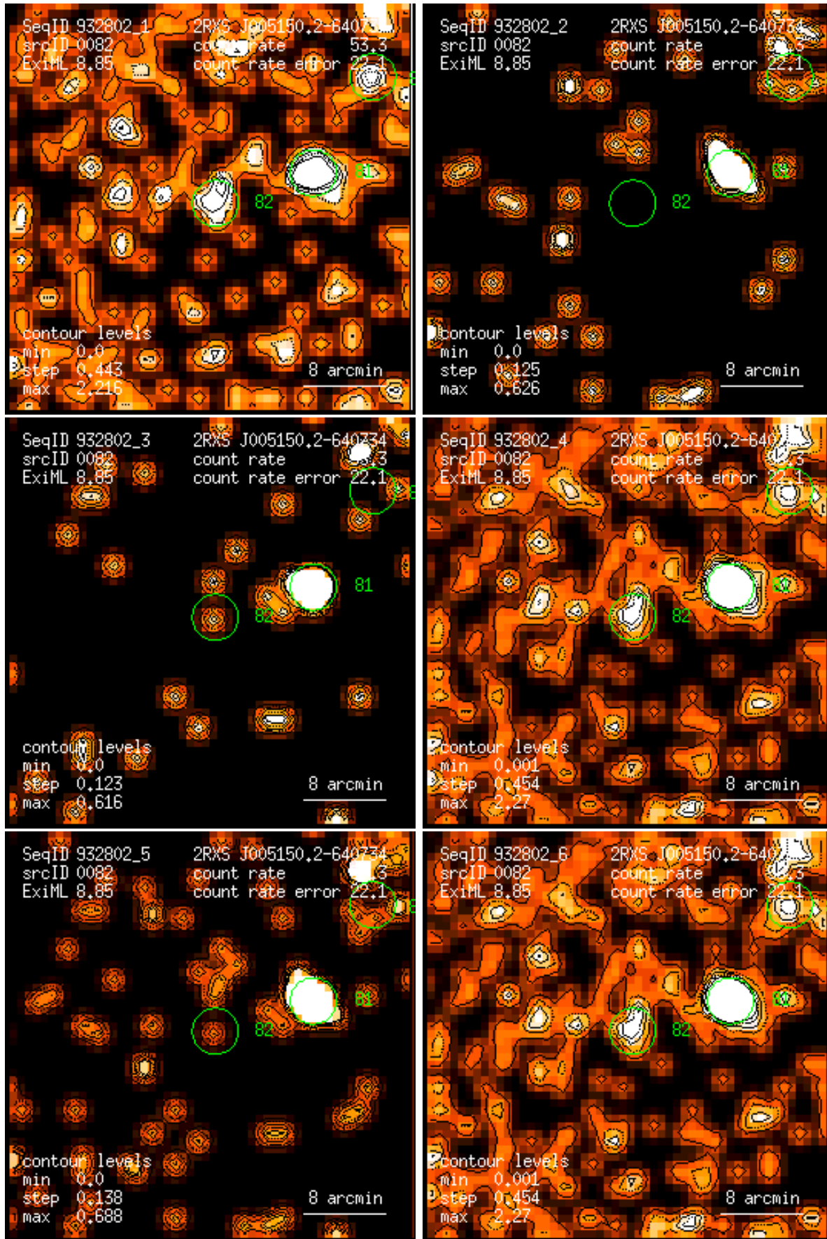
Figure 82: RASS 932802: detection 0082: band rate images, Gaussian filter: (1) PSPC channels 11 – 41, (2) 52 – 90, (3) 91 – 201, (4) 11 – 235, (5) 52 – 201, (6) 11 – 201. Broad band rates in counts/ks. Band rate contour levels in counts/ks/arcmin 2 .
