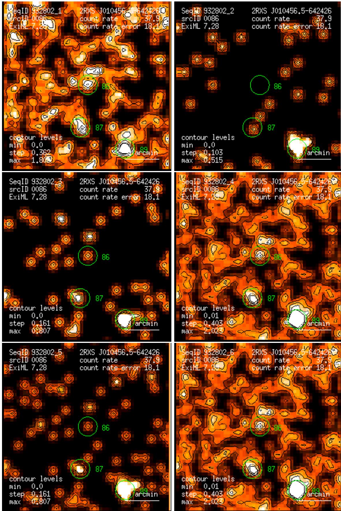
Figure 86: RASS 932802: detection 0086: band rate images, Gaussian filter: (1) PSPC channels 11 – 41, (2) 52 – 90, (3) 91 – 201, (4) 11 – 235, (5) 52 – 201, (6) 11 – 201. Broad band rates in counts/ks. Band rate contour levels in counts/ks/arcmin 2 .
