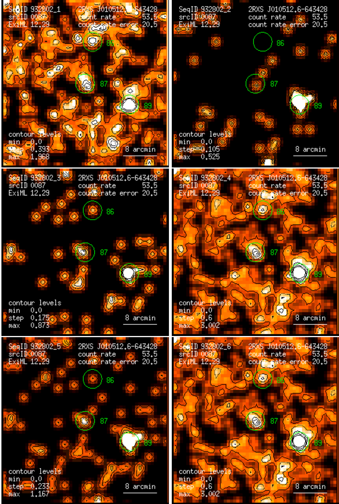
Figure 87: RASS 932802: detection 0087: band rate images, Gaussian filter: (1) PSPC channels 11 – 41, (2) 52 – 90, (3) 91 – 201, (4) 11 – 235, (5) 52 – 201, (6) 11 – 201. Broad band rates in counts/ks. Band rate contour levels in counts/ks/arcmin 2 .
