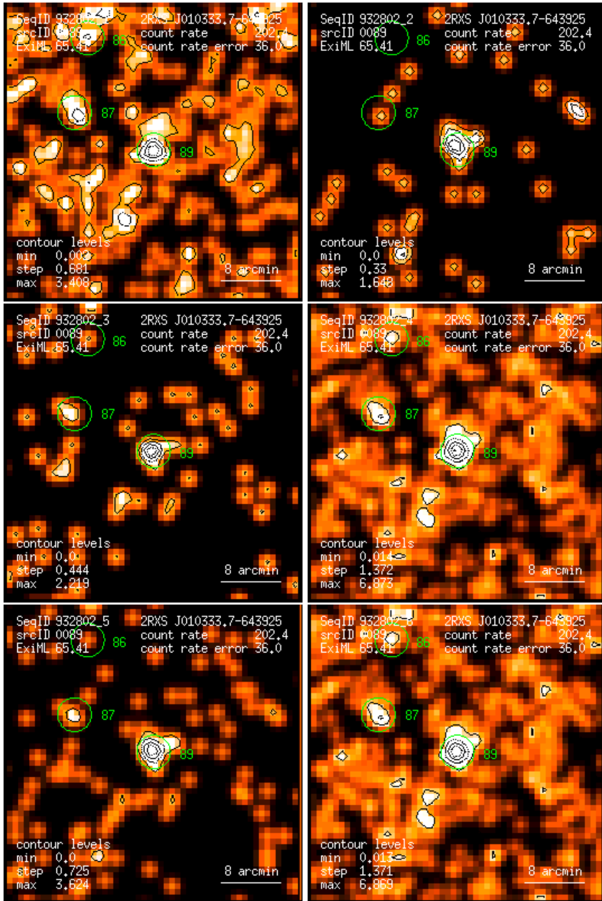
Figure 89: RASS 932802: detection 0089: band rate images, Gaussian filter: (1) PSPC channels 11 – 41, (2) 52 – 90, (3) 91 – 201, (4) 11 – 235, (5) 52 – 201, (6) 11 – 201. Broad band rates in counts/ks. Band rate contour levels in counts/ks/arcmin 2 .
