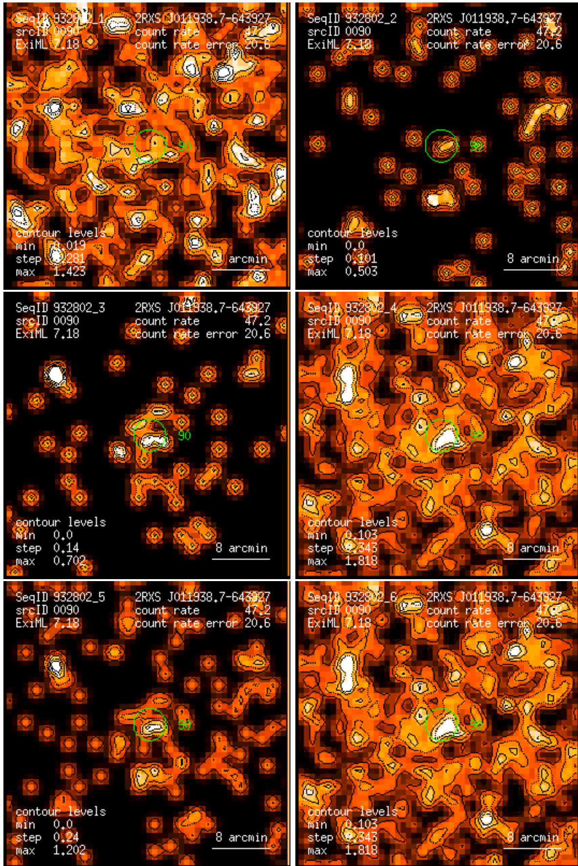
Figure 90: RASS 932802: detection 0090: band rate images, Gaussian filter: (1) PSPC channels 11 – 41, (2) 52 – 90, (3) 91 – 201, (4) 11 – 235, (5) 52 – 201, (6) 11 – 201. Broad band rates in counts/ks. Band rate contour levels in counts/ks/arcmin 2 .
