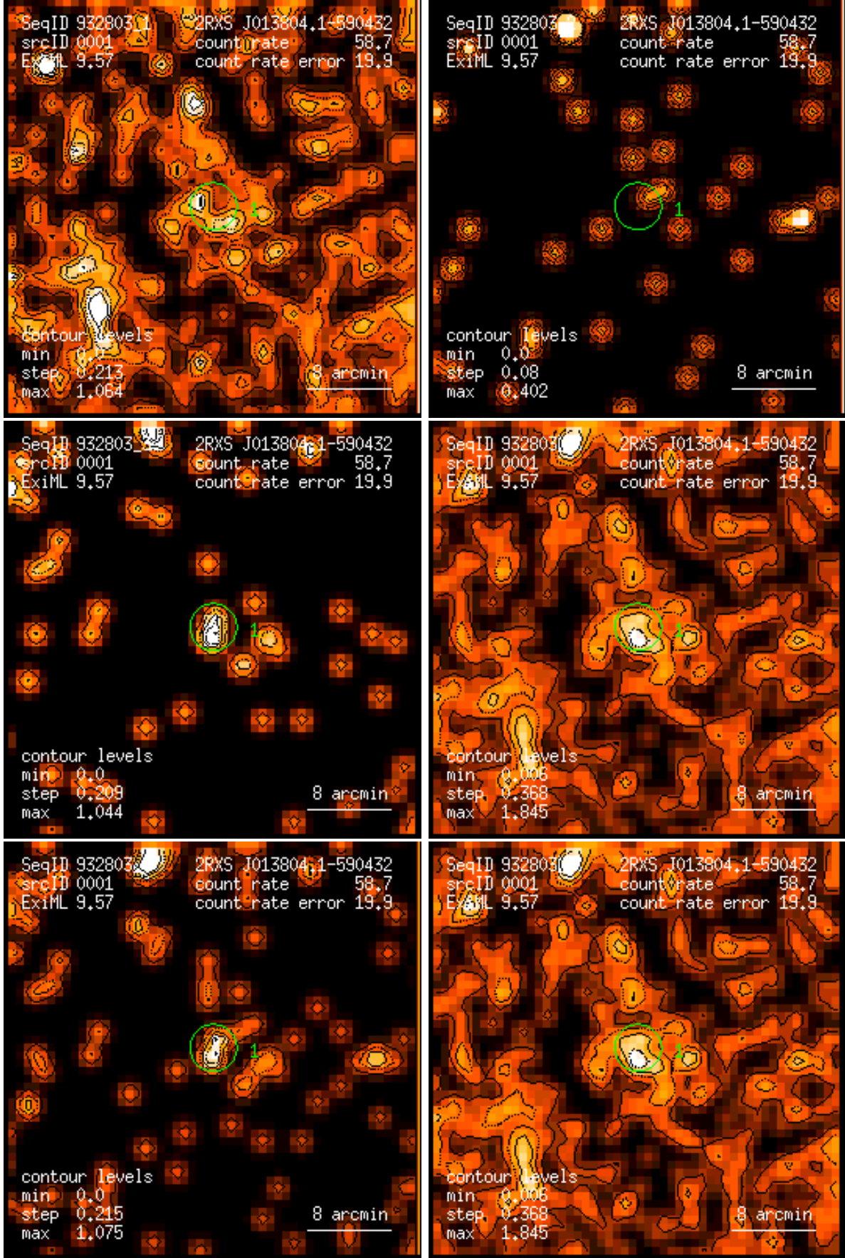
Figure 1: RASS 932803: detection 0001: band rate images, Gaussian filter: (1) PSPC channels 11 – 41, (2) 52 – 90, (3) 91 – 201, (4) 11 – 235, (5) 52 – 201, (6) 11 – 201. Broad band rates in counts/ks. Band rate contour levels in counts/ks/arcmin 2 .
