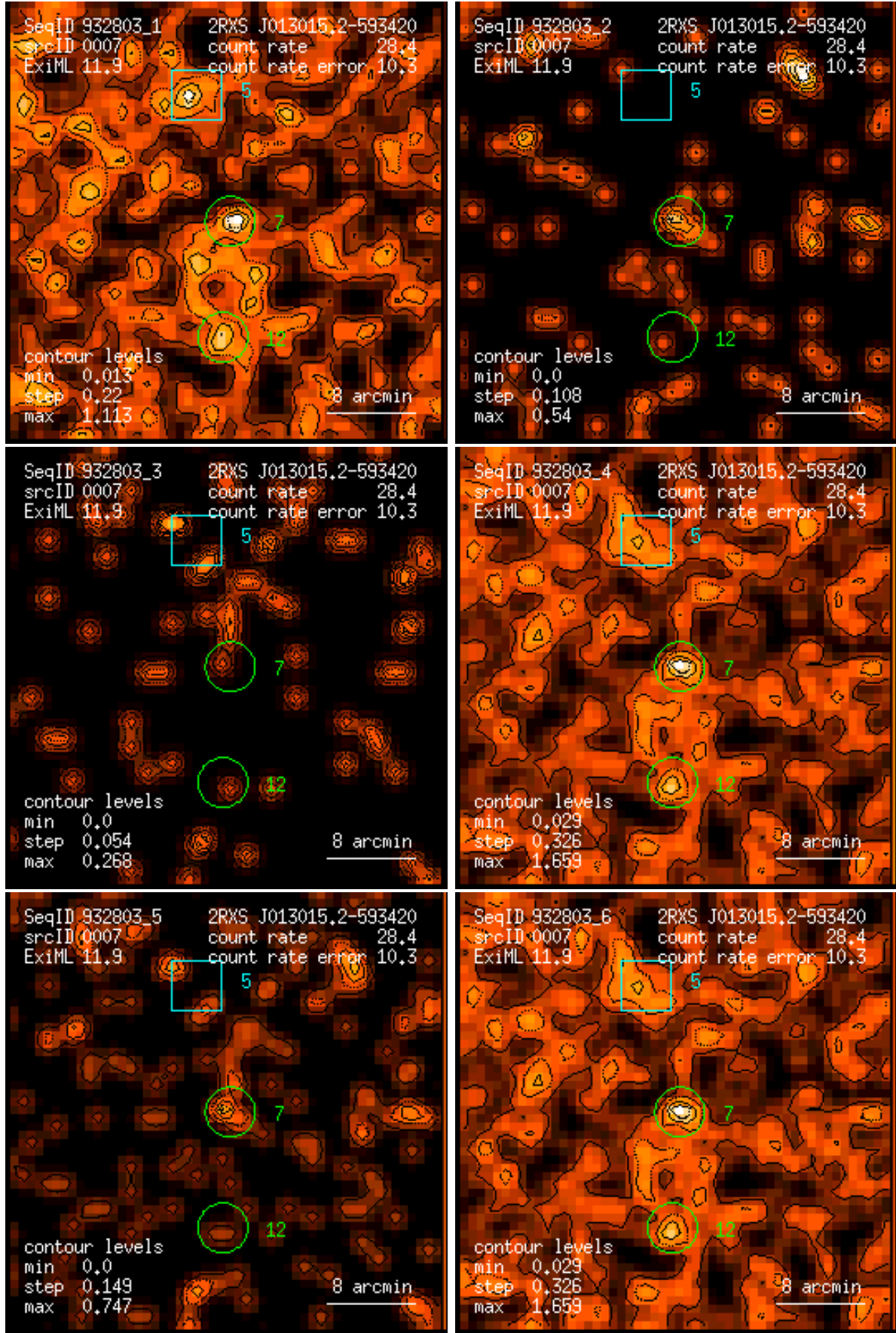
Figure 7: RASS 932803: detection 0007: band rate images, Gaussian filter: (1) PSPC channels 11 – 41, (2) 52 – 90, (3) 91 – 201, (4) 11 – 235, (5) 52 – 201, (6) 11 – 201. Broad band rates in counts/ks. Band rate contour levels in counts/ks/arcmin 2 .
