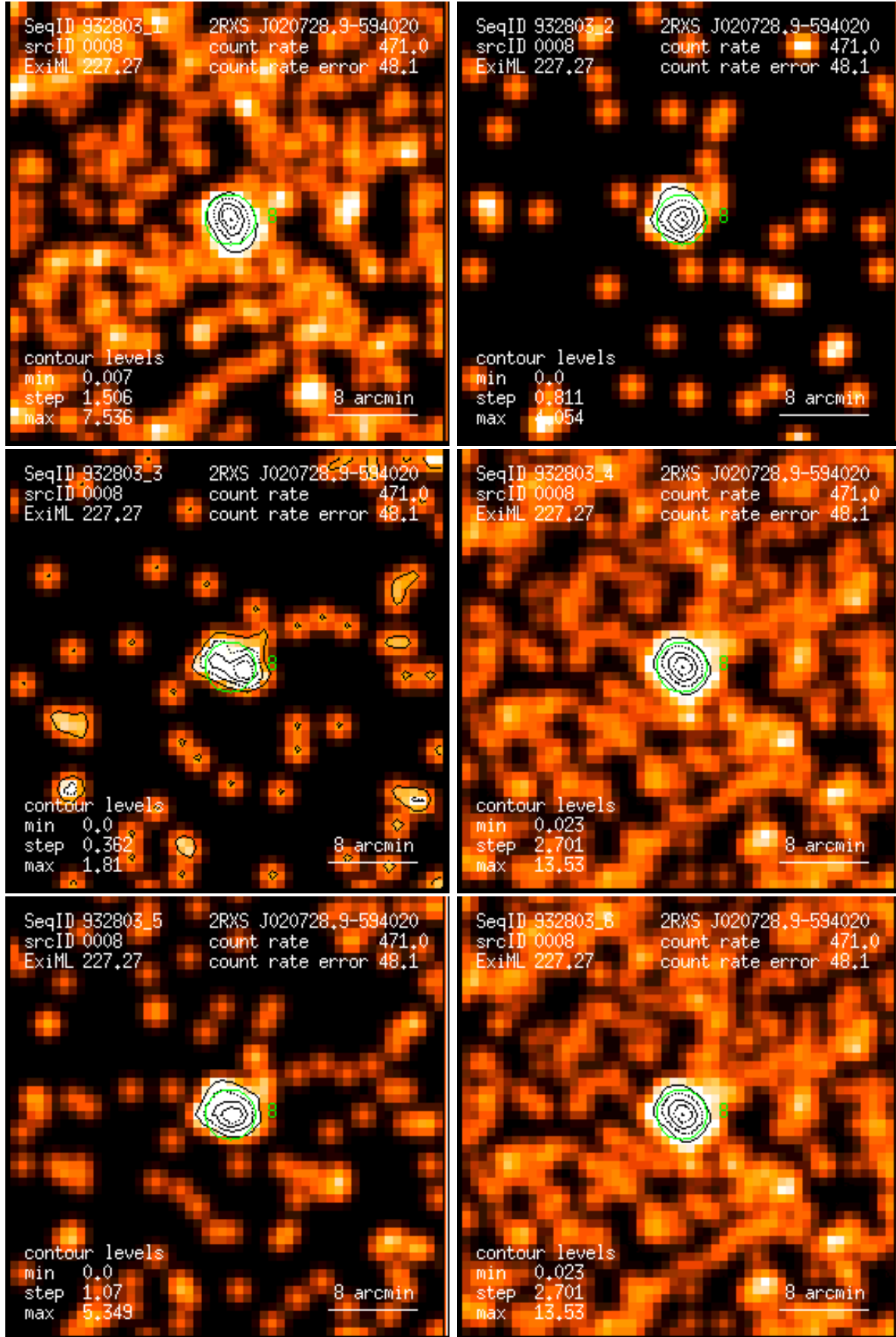
Figure 8: RASS 932803: detection 0008: band rate images, Gaussian filter: (1) PSPC channels 11 – 41, (2) 52 – 90, (3) 91 – 201, (4) 11 – 235, (5) 52 – 201, (6) 11 – 201. Broad band rates in counts/ks. Band rate contour levels in counts/ks/arcmin 2 .
