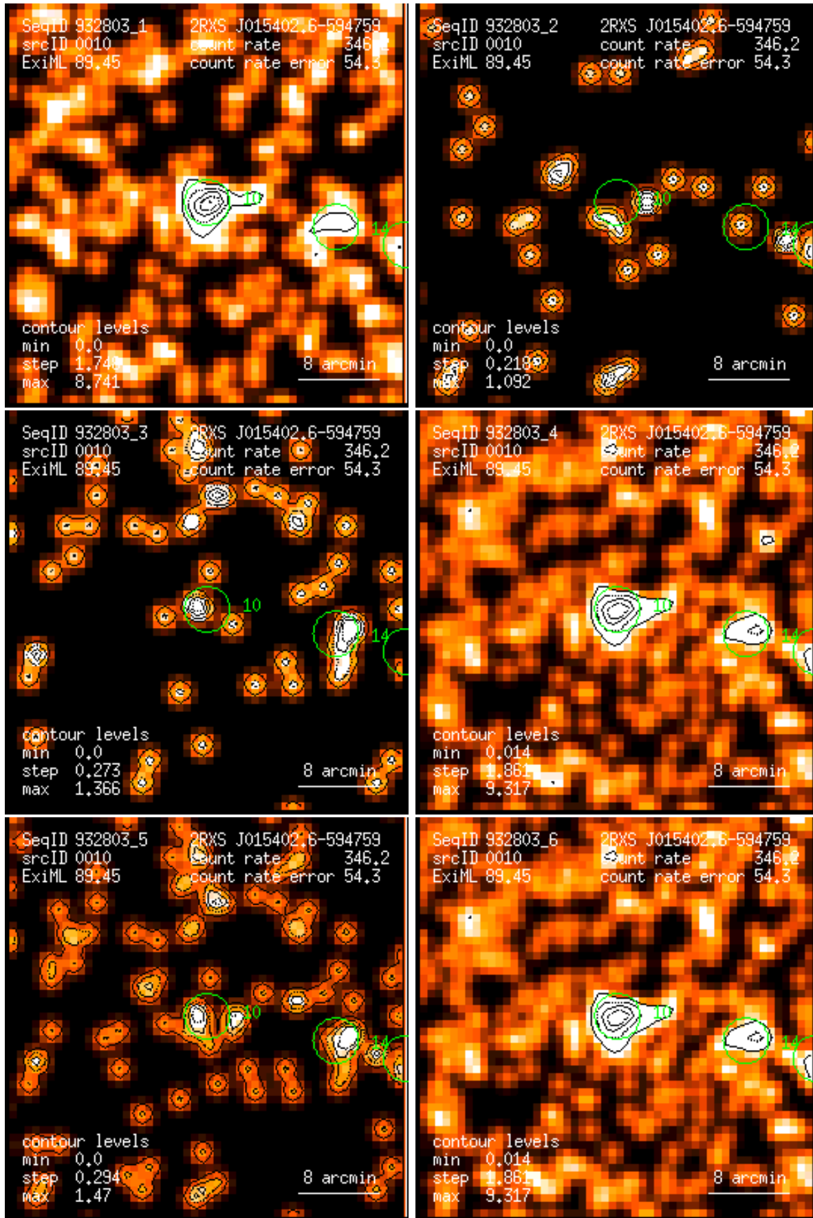
Figure 10: RASS 932803: detection 0010: band rate images, Gaussian filter: (1) PSPC channels 11 – 41, (2) 52 – 90, (3) 91 – 201, (4) 11 – 235, (5) 52 – 201, (6) 11 – 201. Broad band rates in counts/ks. Band rate contour levels in counts/ks/arcmin 2 .
