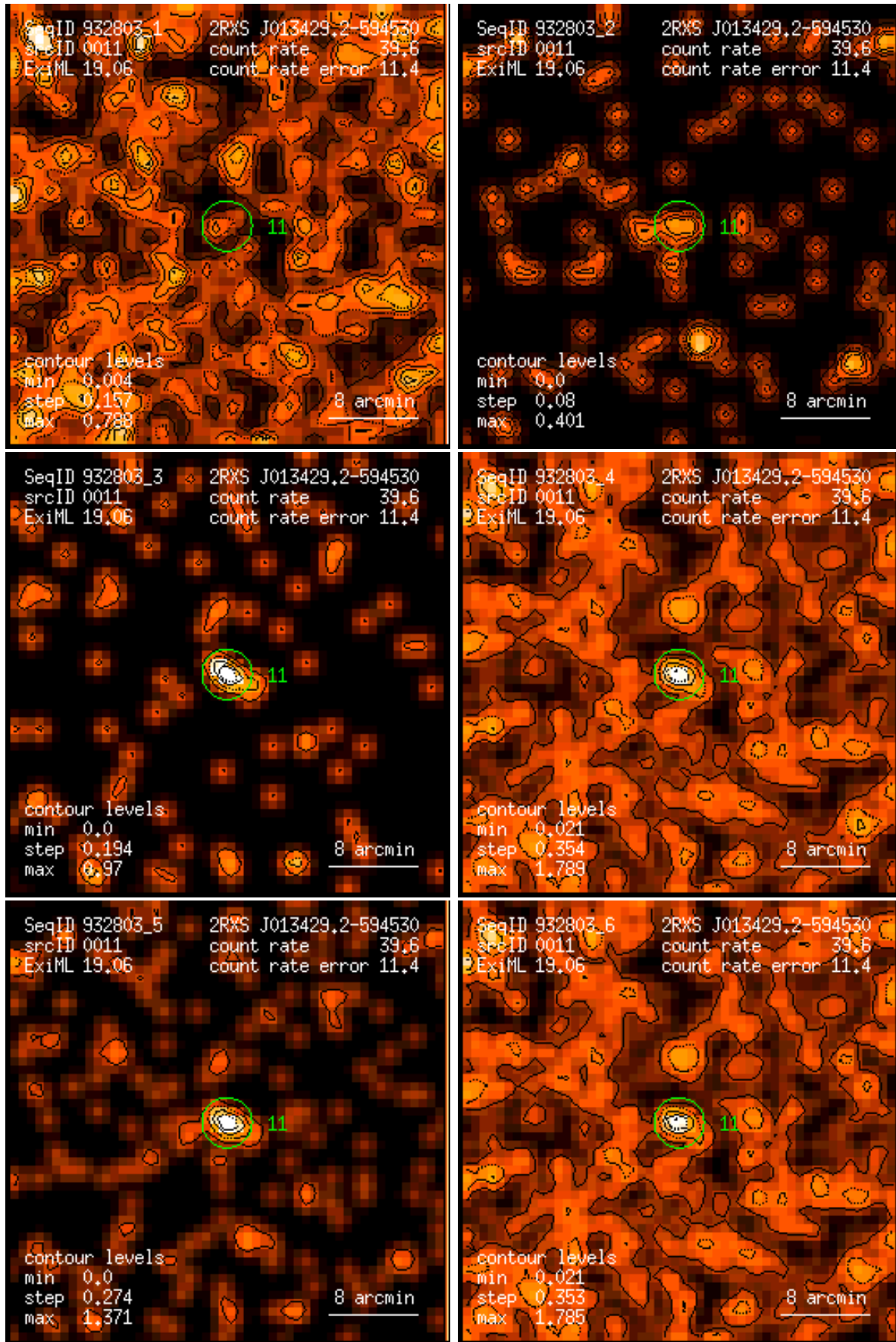
Figure 11: RASS 932803: detection 0011: band rate images, Gaussian filter: (1) PSPC channels 11 – 41, (2) 52 – 90, (3) 91 – 201, (4) 11 – 235, (5) 52 – 201, (6) 11 – 201. Broad band rates in counts/ks. Band rate contour levels in counts/ks/arcmin 2 .
