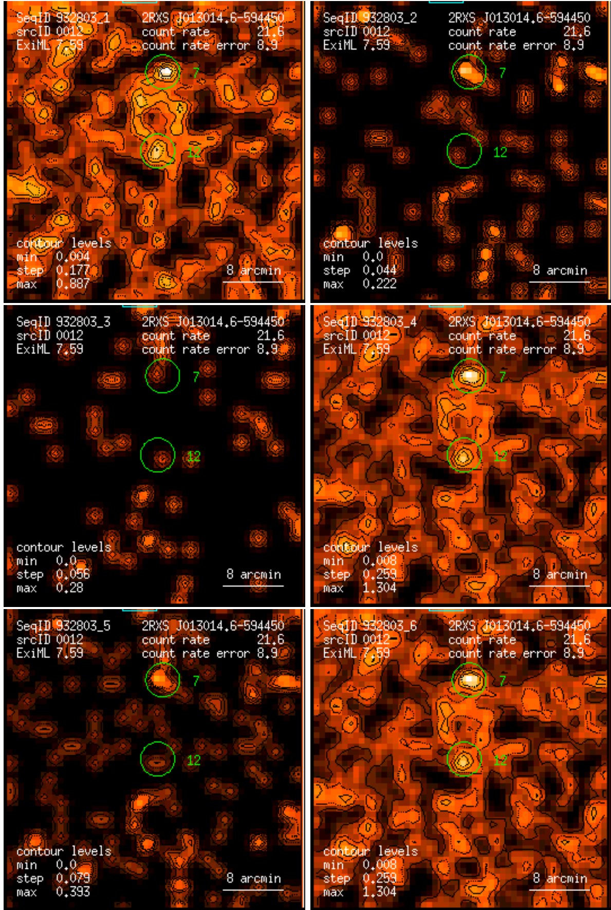
Figure 12: RASS 932803: detection 0012: band rate images, Gaussian filter: (1) PSPC channels 11 – 41, (2) 52 – 90, (3) 91 – 201, (4) 11 – 235, (5) 52 – 201, (6) 11 – 201. Broad band rates in counts/ks. Band rate contour levels in counts/ks/arcmin 2 .
