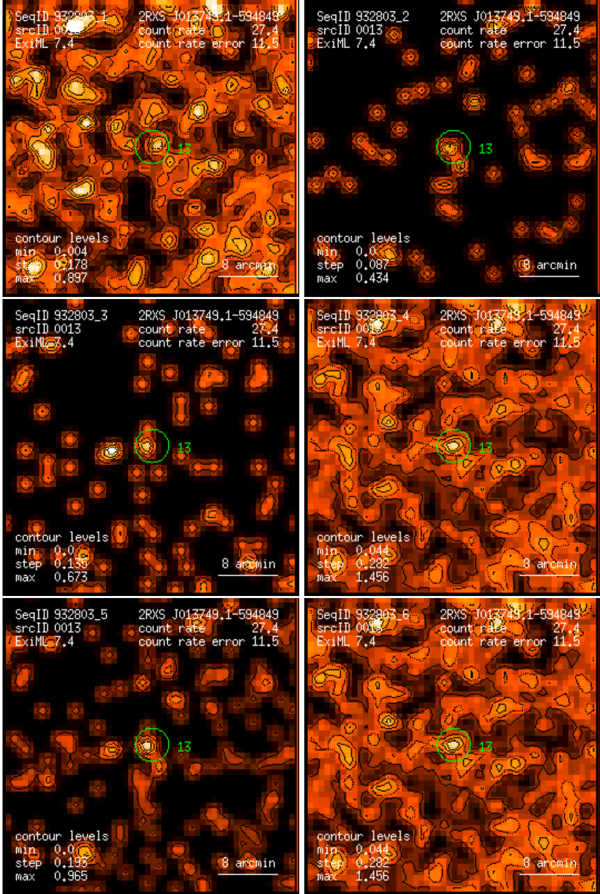
Figure 13: RASS 932803: detection 0013: band rate images, Gaussian filter: (1) PSPC channels 11 – 41, (2) 52 – 90, (3) 91 – 201, (4) 11 – 235, (5) 52 – 201, (6) 11 – 201. Broad band rates in counts/ks. Band rate contour levels in counts/ks/arcmin 2 .
