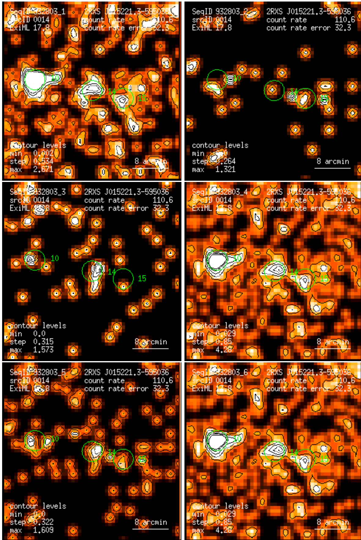
Figure 14: RASS 932803: detection 0014: band rate images, Gaussian filter: (1) PSPC channels 11 – 41, (2) 52 – 90, (3) 91 – 201, (4) 11 – 235, (5) 52 – 201, (6) 11 – 201. Broad band rates in counts/ks. Band rate contour levels in counts/ks/arcmin 2 .
