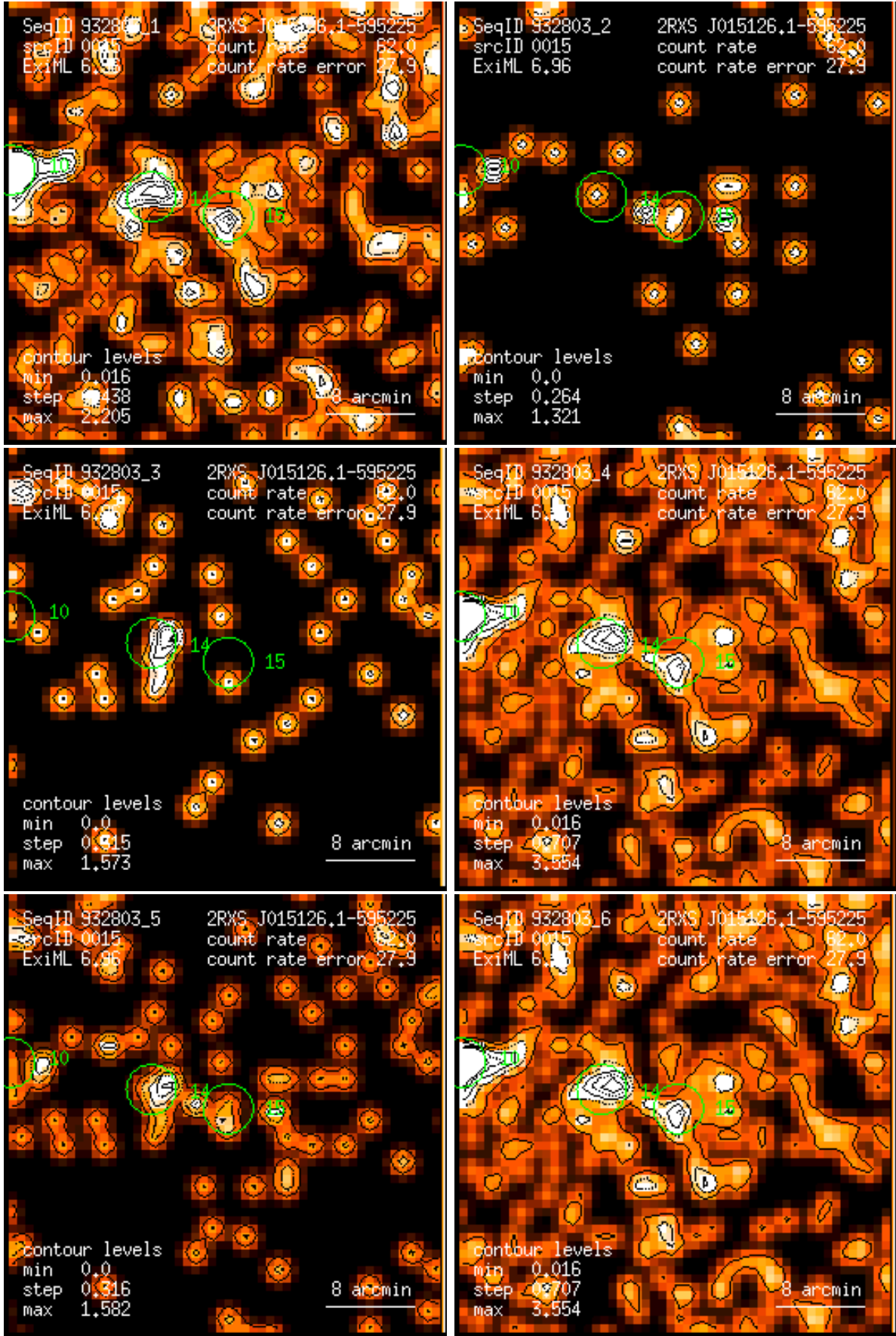
Figure 15: RASS 932803: detection 0015: band rate images, Gaussian filter: (1) PSPC channels 11 – 41, (2) 52 – 90, (3) 91 – 201, (4) 11 – 235, (5) 52 – 201, (6) 11 – 201. Broad band rates in counts/ks. Band rate contour levels in counts/ks/arcmin 2 .
