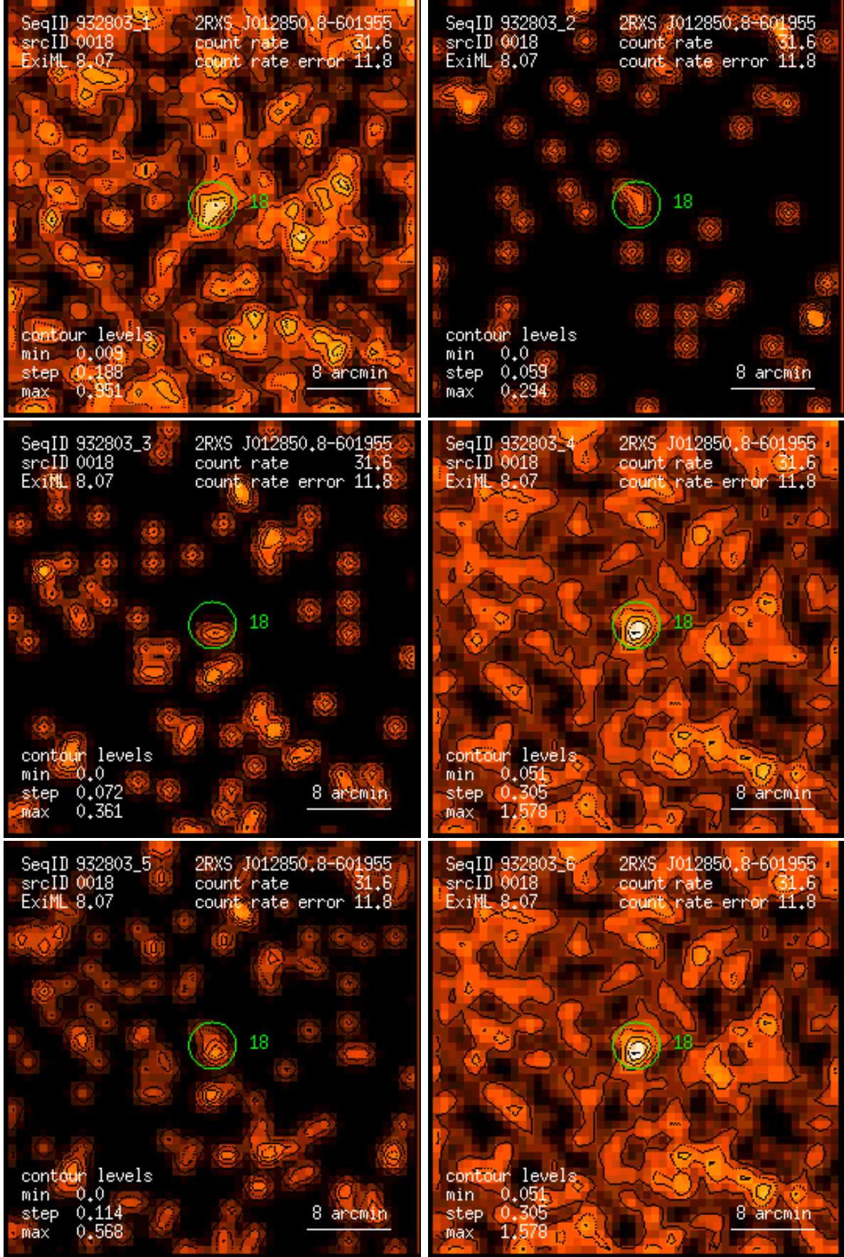
Figure 18: RASS 932803: detection 0018: band rate images, Gaussian filter: (1) PSPC channels 11 – 41, (2) 52 – 90, (3) 91 – 201, (4) 11 – 235, (5) 52 – 201, (6) 11 – 201. Broad band rates in counts/ks. Band rate contour levels in counts/ks/arcmin 2 .
