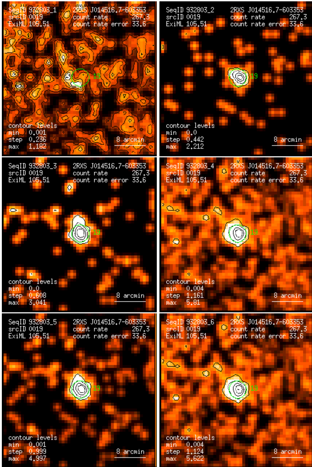
Figure 19: RASS 932803: detection 0019: band rate images, Gaussian filter: (1) PSPC channels 11 – 41, (2) 52 – 90, (3) 91 – 201, (4) 11 – 235, (5) 52 – 201, (6) 11 – 201. Broad band rates in counts/ks. Band rate contour levels in counts/ks/arcmin 2 .
