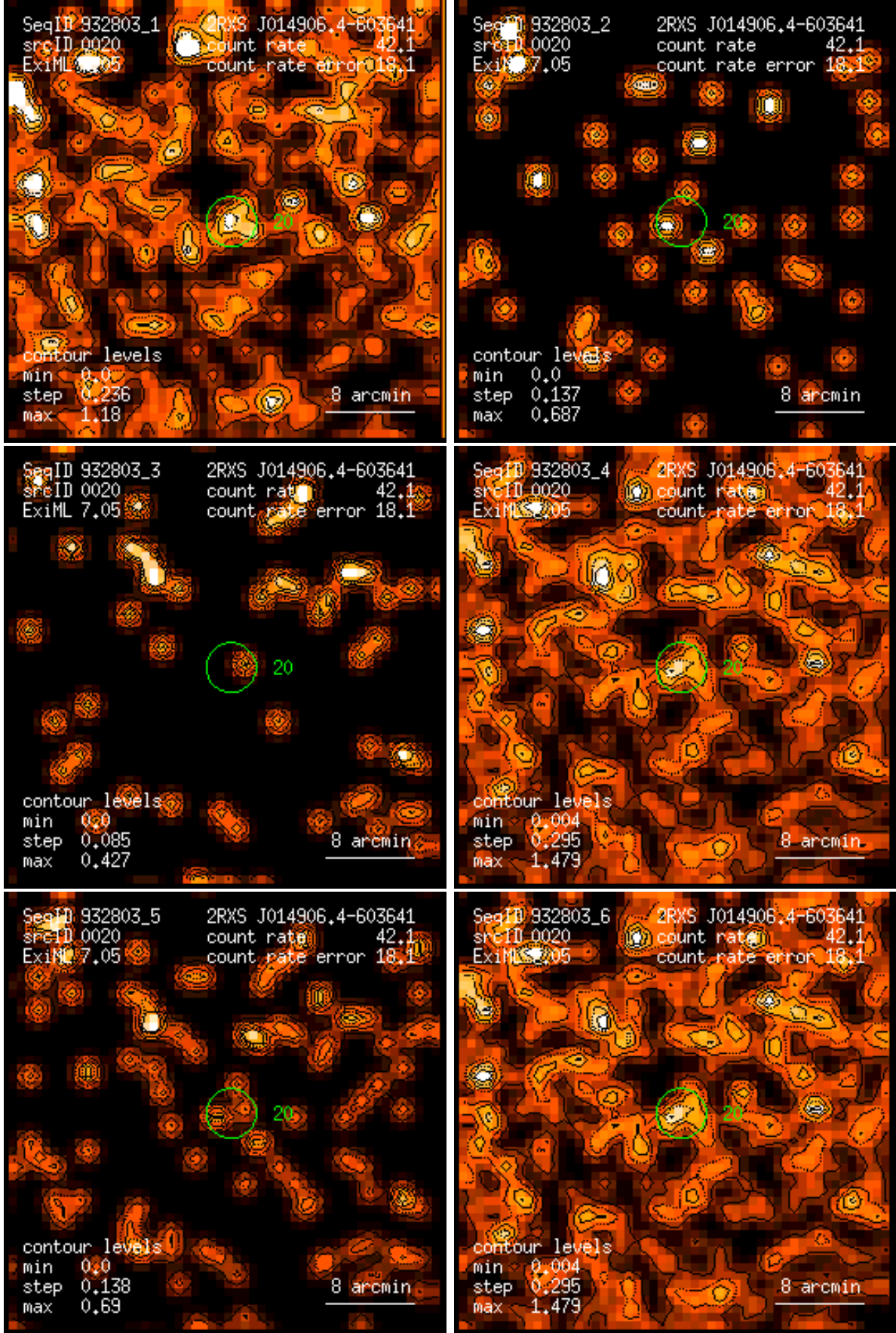
Figure 20: RASS 932803: detection 0020: band rate images, Gaussian filter: (1) PSPC channels 11 – 41, (2) 52 – 90, (3) 91 – 201, (4) 11 – 235, (5) 52 – 201, (6) 11 – 201. Broad band rates in counts/ks. Band rate contour levels in counts/ks/arcmin 2 .
