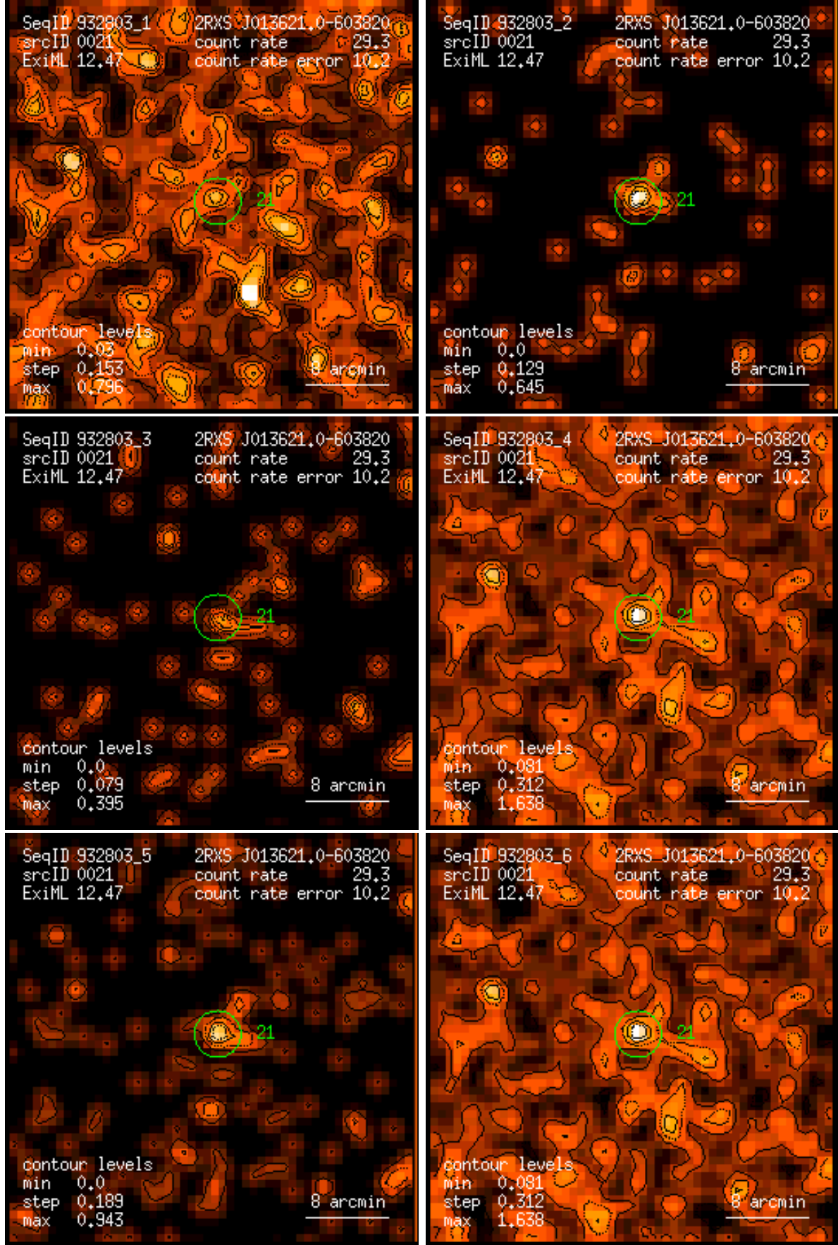
Figure 21: RASS 932803: detection 0021: band rate images, Gaussian filter: (1) PSPC channels 11 – 41, (2) 52 – 90, (3) 91 – 201, (4) 11 – 235, (5) 52 – 201, (6) 11 – 201. Broad band rates in counts/ks. Band rate contour levels in counts/ks/arcmin 2 .
