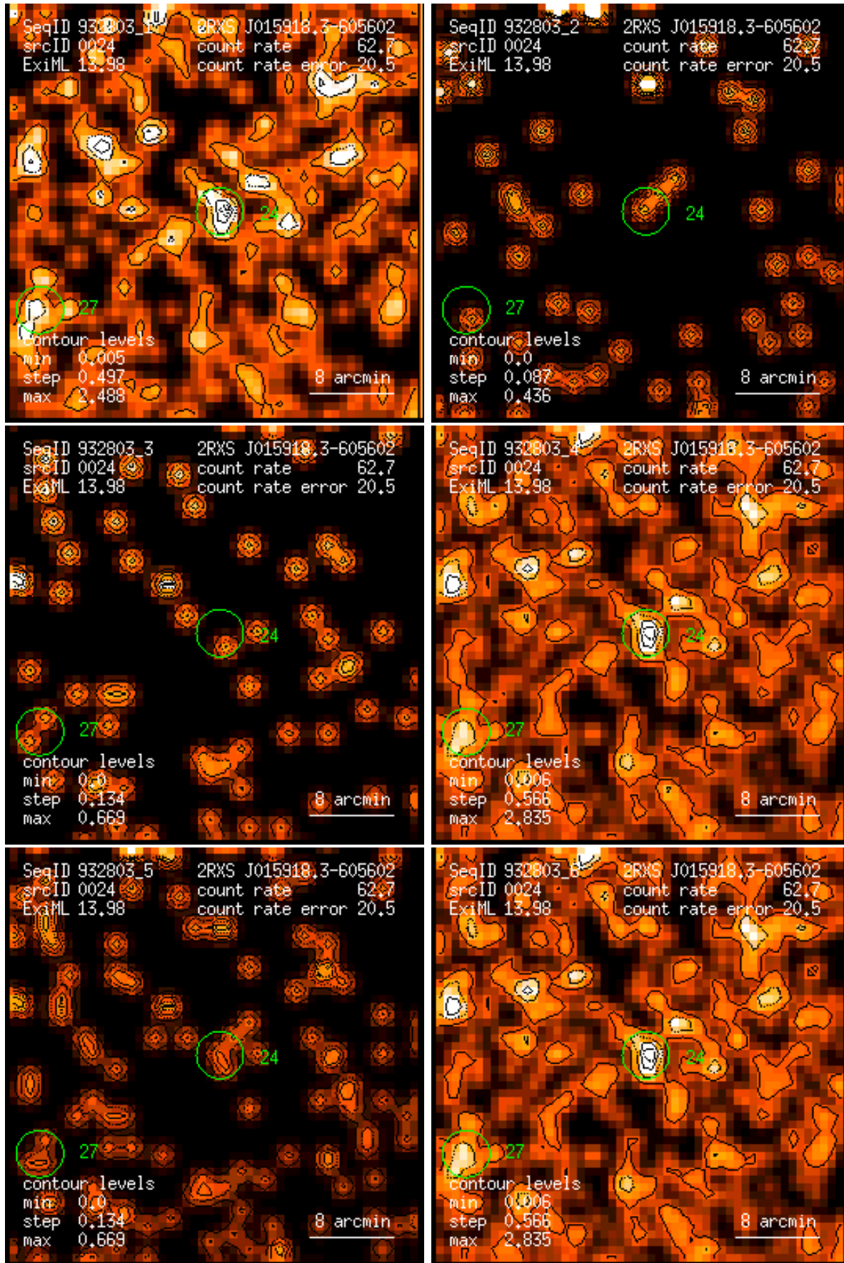
Figure 24: RASS 932803: detection 0024: band rate images, Gaussian filter: (1) PSPC channels 11 – 41, (2) 52 – 90, (3) 91 – 201, (4) 11 – 235, (5) 52 – 201, (6) 11 – 201. Broad band rates in counts/ks. Band rate contour levels in counts/ks/arcmin 2 .
