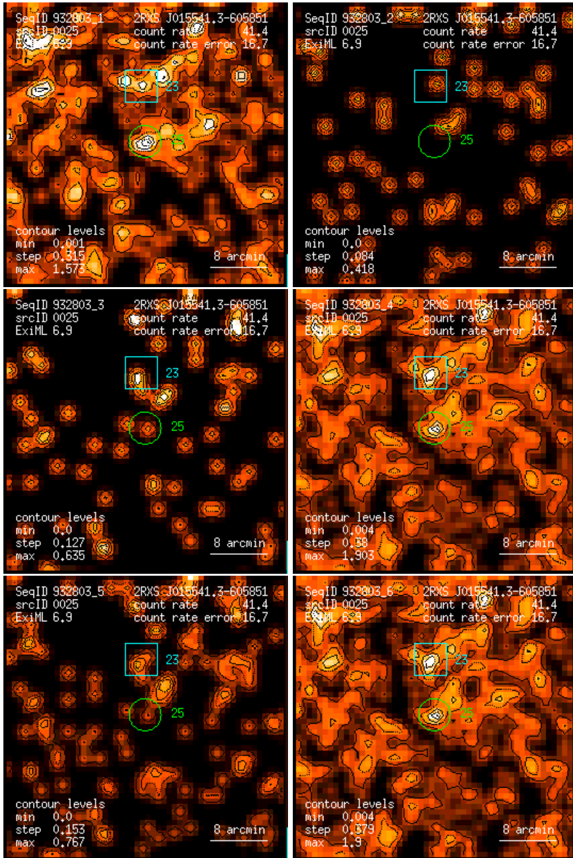
Figure 25: RASS 932803: detection 0025: band rate images, Gaussian filter: (1) PSPC channels 11 – 41, (2) 52 – 90, (3) 91 – 201, (4) 11 – 235, (5) 52 – 201, (6) 11 – 201. Broad band rates in counts/ks. Band rate contour levels in counts/ks/arcmin 2 .
