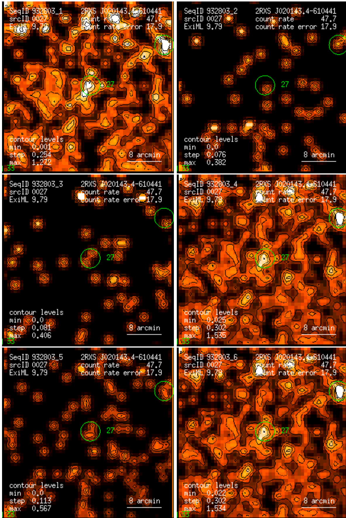
Figure 27: RASS 932803: detection 0027: band rate images, Gaussian filter: (1) PSPC channels 11 – 41, (2) 52 – 90, (3) 91 – 201, (4) 11 – 235, (5) 52 – 201, (6) 11 – 201. Broad band rates in counts/ks. Band rate contour levels in counts/ks/arcmin 2 .
