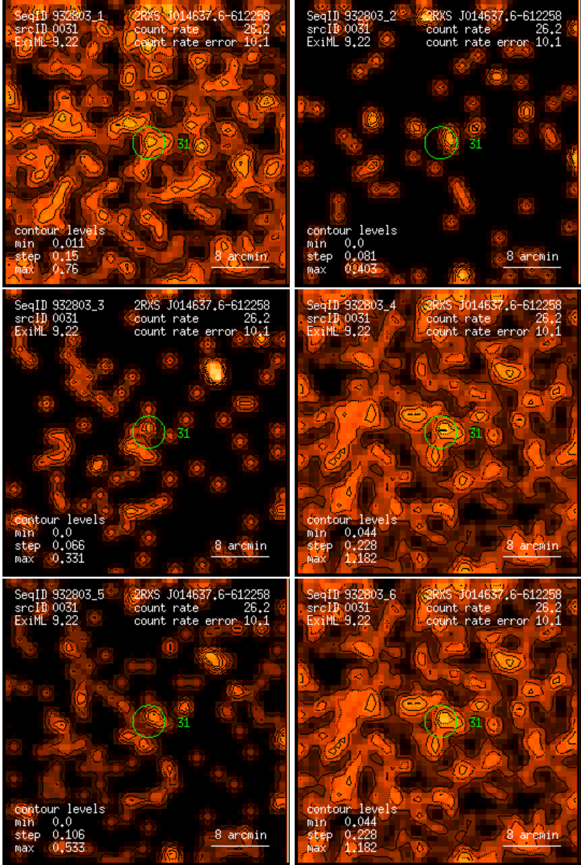
Figure 31: RASS 932803: detection 0031: band rate images, Gaussian filter: (1) PSPC channels 11 – 41, (2) 52 – 90, (3) 91 – 201, (4) 11 – 235, (5) 52 – 201, (6) 11 – 201. Broad band rates in counts/ks. Band rate contour levels in counts/ks/arcmin 2 .
