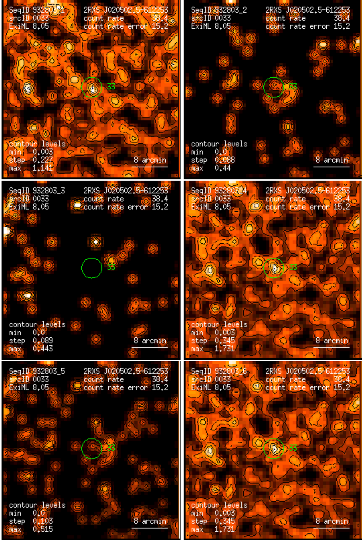
Figure 33: RASS 932803: detection 0033: band rate images, Gaussian filter: (1) PSPC channels 11 – 41, (2) 52 – 90, (3) 91 – 201, (4) 11 – 235, (5) 52 – 201, (6) 11 – 201. Broad band rates in counts/ks. Band rate contour levels in counts/ks/arcmin 2 .
