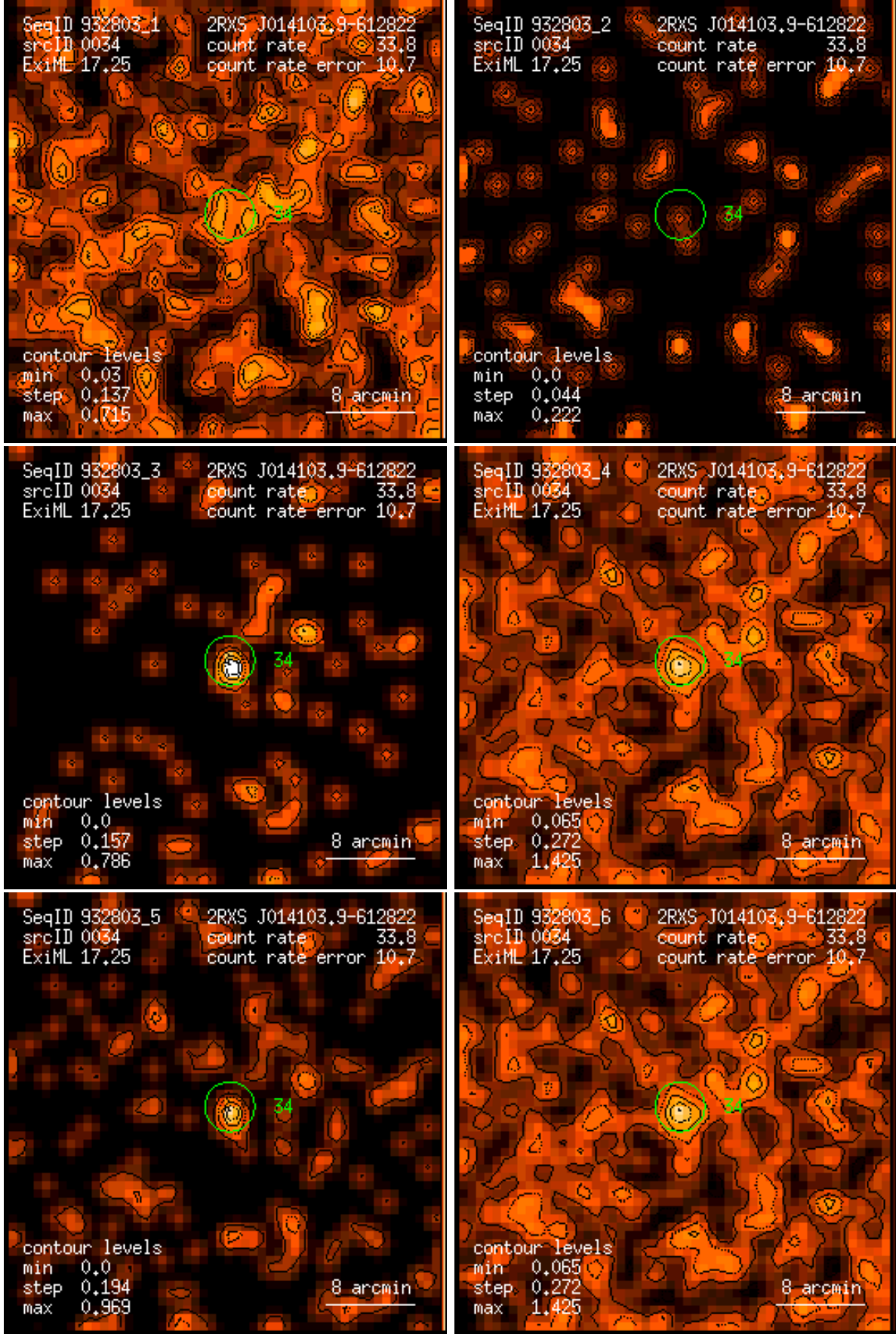
Figure 34: RASS 932803: detection 0034: band rate images, Gaussian filter: (1) PSPC channels 11 – 41, (2) 52 – 90, (3) 91 – 201, (4) 11 – 235, (5) 52 – 201, (6) 11 – 201. Broad band rates in counts/ks. Band rate contour levels in counts/ks/arcmin 2 .
