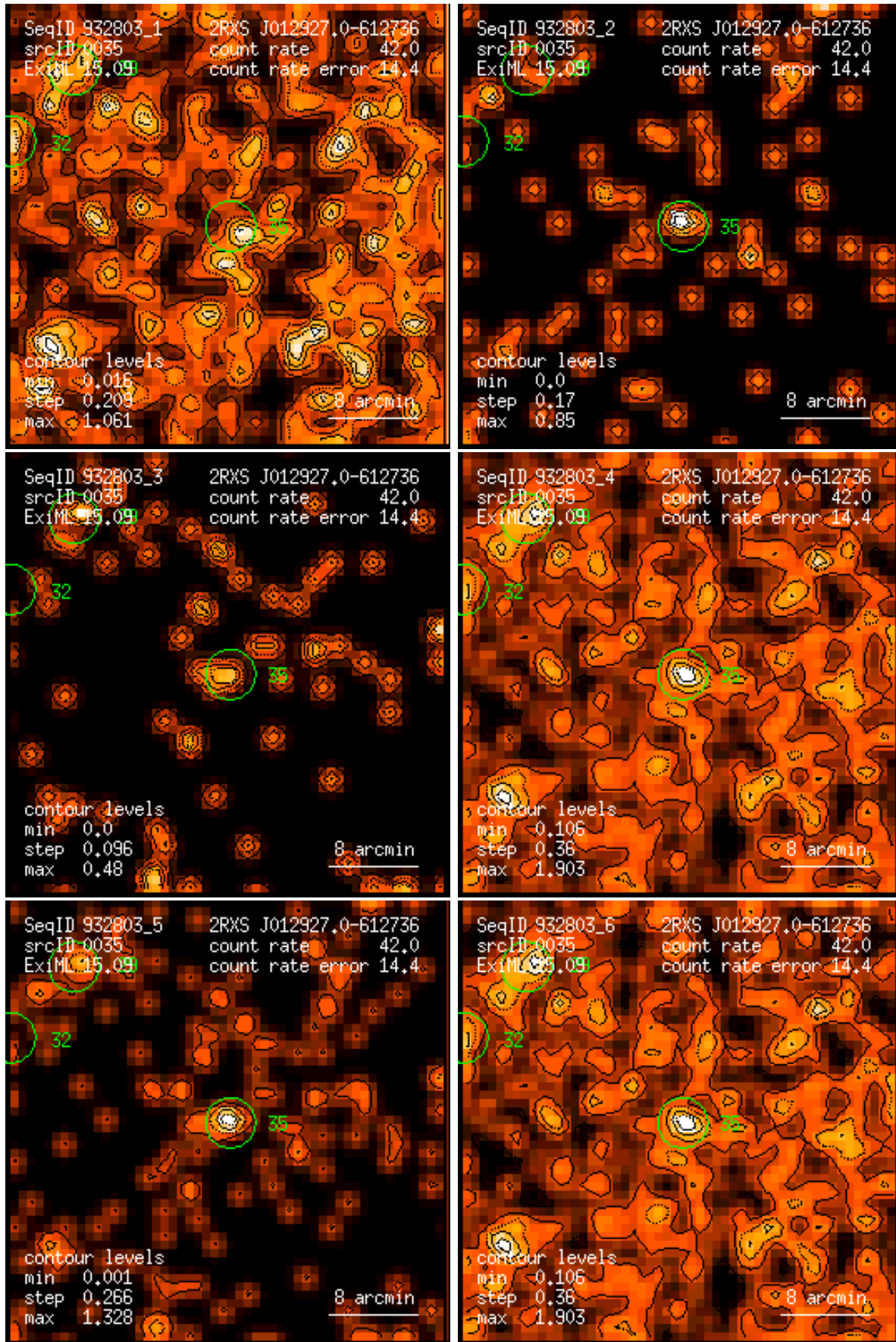
Figure 35: RASS 932803: detection 0035: band rate images, Gaussian filter: (1) PSPC channels 11 – 41, (2) 52 – 90, (3) 91 – 201, (4) 11 – 235, (5) 52 – 201, (6) 11 – 201. Broad band rates in counts/ks. Band rate contour levels in counts/ks/arcmin 2 .
