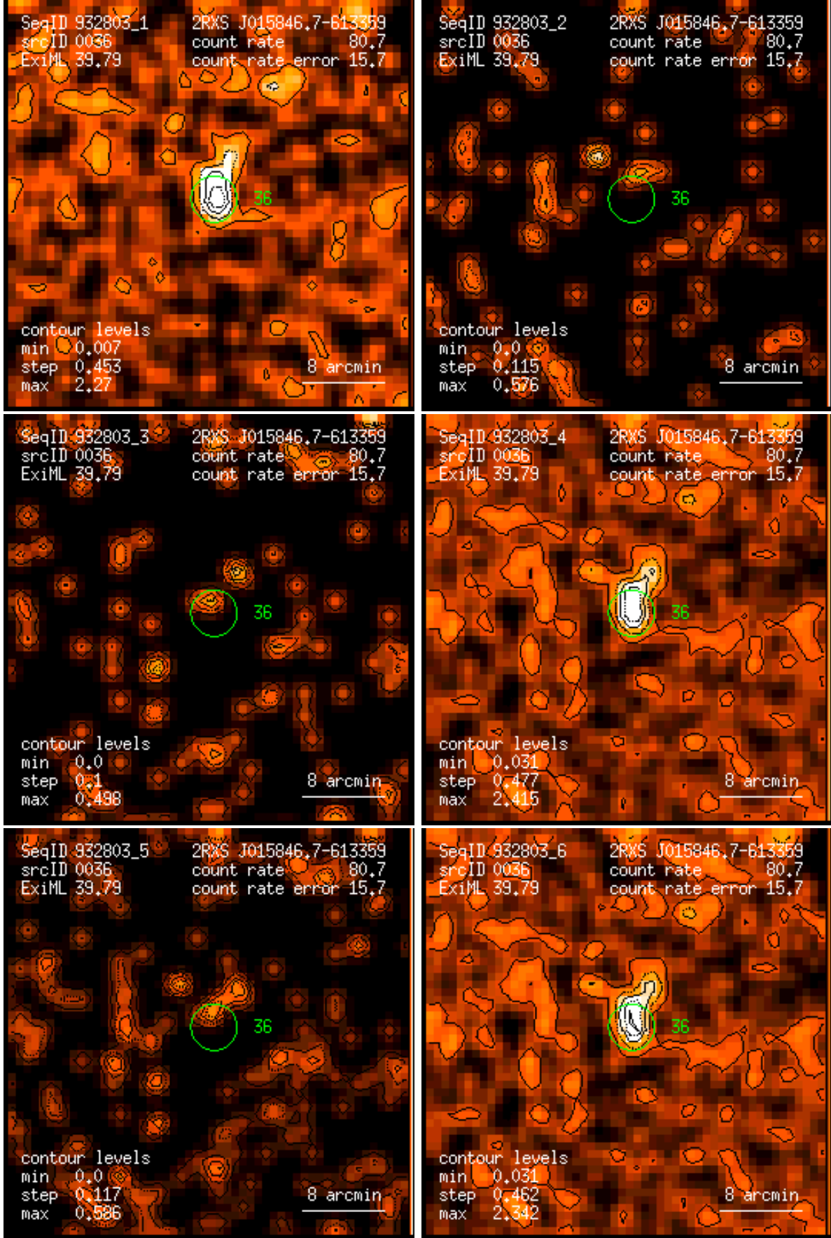
Figure 36: RASS 932803: detection 0036: band rate images, Gaussian filter: (1) PSPC channels 11 – 41, (2) 52 – 90, (3) 91 – 201, (4) 11 – 235, (5) 52 – 201, (6) 11 – 201. Broad band rates in counts/ks. Band rate contour levels in counts/ks/arcmin 2 .
