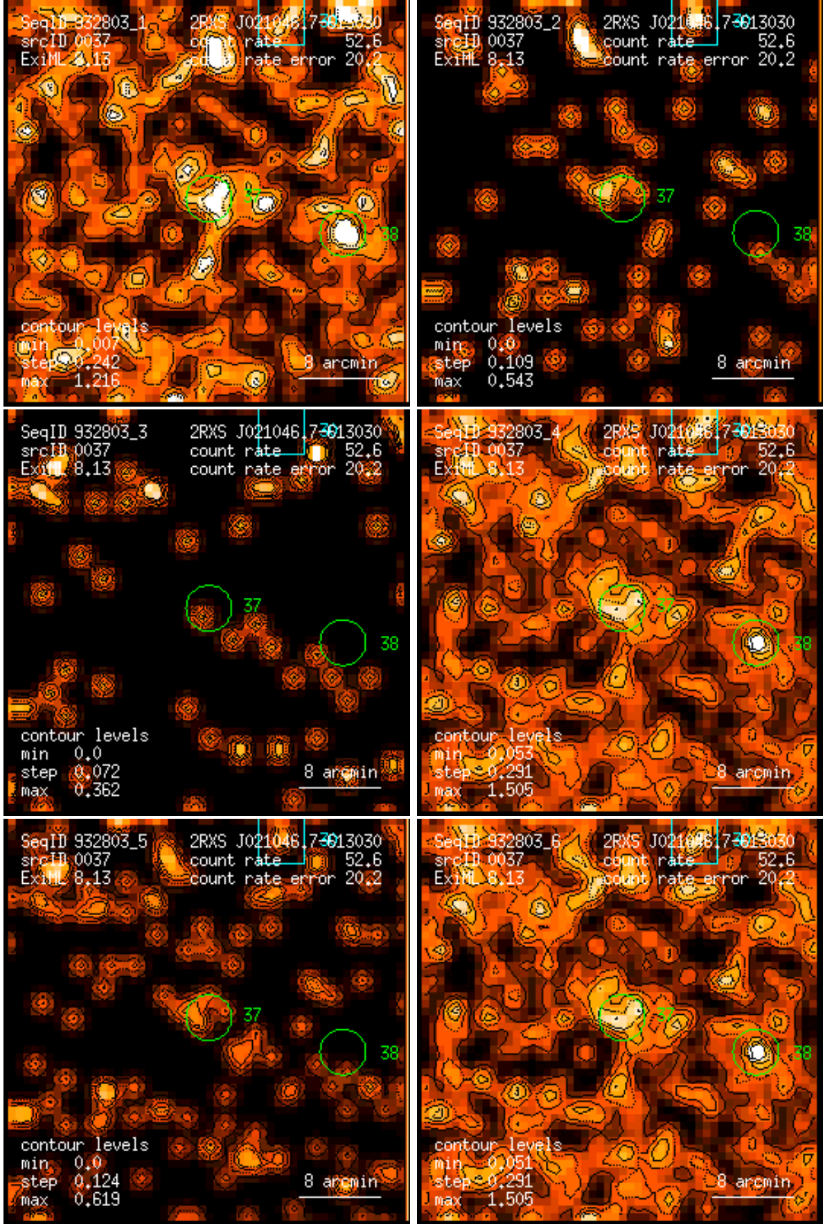
Figure 37: RASS 932803: detection 0037: band rate images, Gaussian filter: (1) PSPC channels 11 – 41, (2) 52 – 90, (3) 91 – 201, (4) 11 – 235, (5) 52 – 201, (6) 11 – 201. Broad band rates in counts/ks. Band rate contour levels in counts/ks/arcmin 2 .
