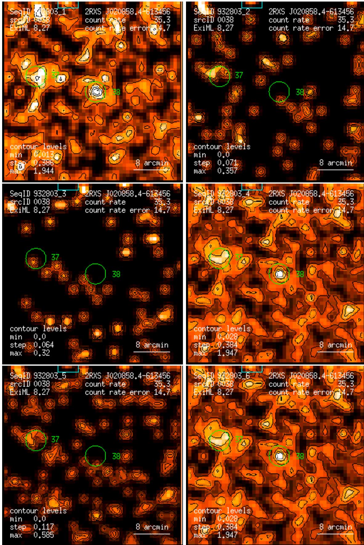
Figure 38: RASS 932803: detection 0038: band rate images, Gaussian filter: (1) PSPC channels 11 – 41, (2) 52 – 90, (3) 91 – 201, (4) 11 – 235, (5) 52 – 201, (6) 11 – 201. Broad band rates in counts/ks. Band rate contour levels in counts/ks/arcmin 2 .
