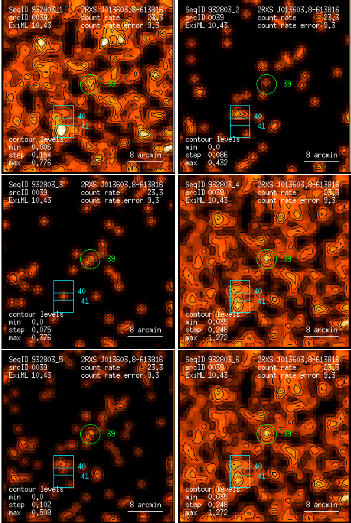
Figure 39: RASS 932803: detection 0039: band rate images, Gaussian filter: (1) PSPC channels 11 – 41, (2) 52 – 90, (3) 91 – 201, (4) 11 – 235, (5) 52 – 201, (6) 11 – 201. Broad band rates in counts/ks. Band rate contour levels in counts/ks/arcmin 2 .
