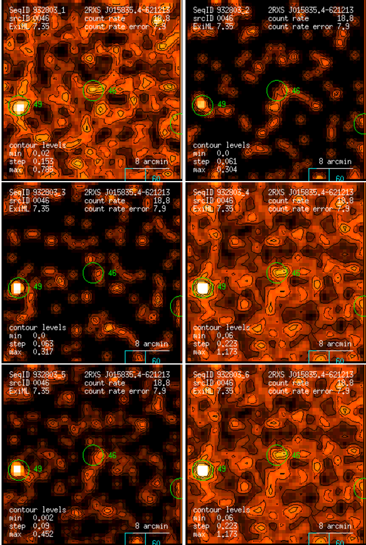
Figure 46: RASS 932803: detection 0046: band rate images, Gaussian filter: (1) PSPC channels 11 – 41, (2) 52 – 90, (3) 91 – 201, (4) 11 – 235, (5) 52 – 201, (6) 11 – 201. Broad band rates in counts/ks. Band rate contour levels in counts/ks/arcmin 2 .
