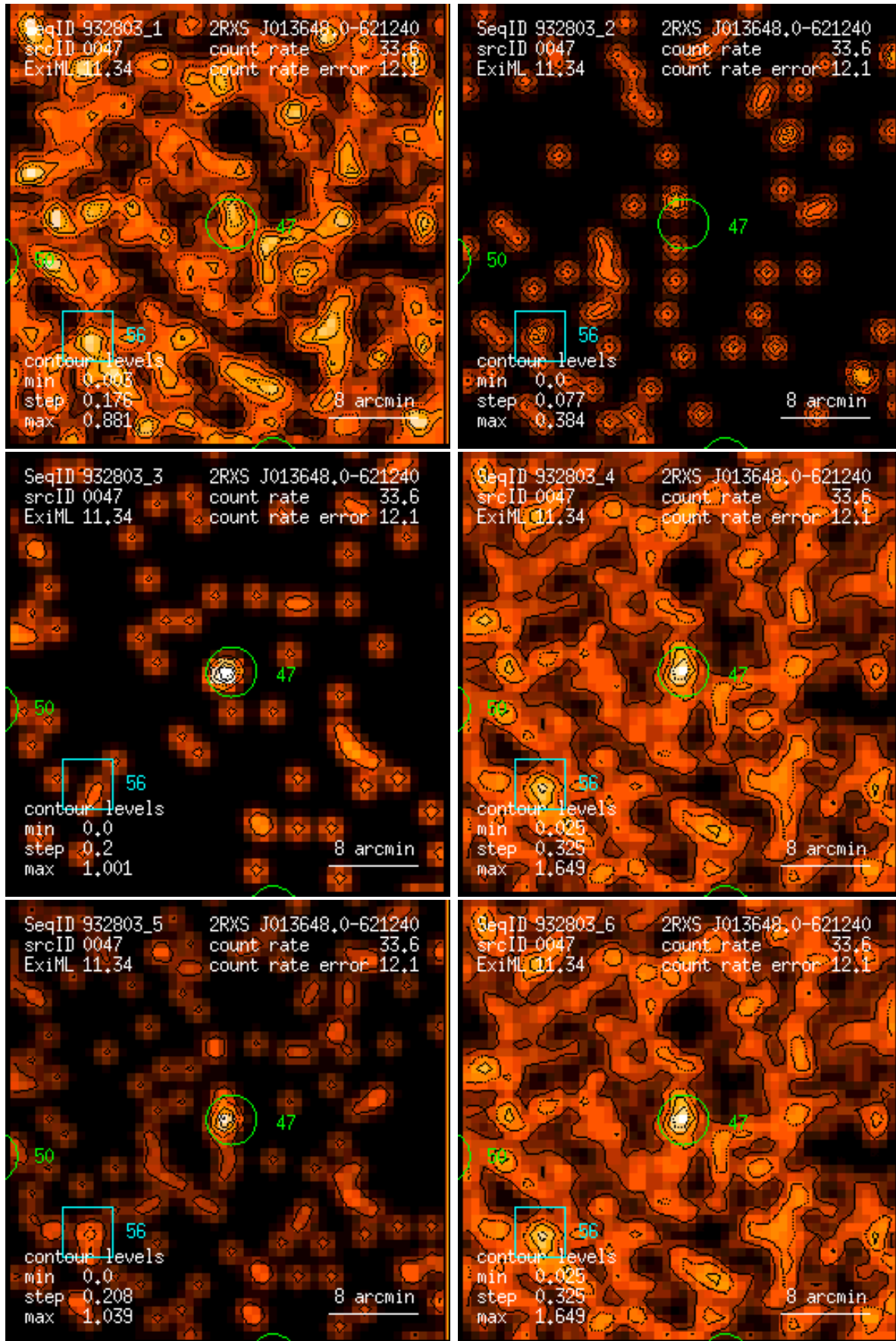
Figure 47: RASS 932803: detection 0047: band rate images, Gaussian filter: (1) PSPC channels 11 – 41, (2) 52 – 90, (3) 91 – 201, (4) 11 – 235, (5) 52 – 201, (6) 11 – 201. Broad band rates in counts/ks. Band rate contour levels in counts/ks/arcmin 2 .
