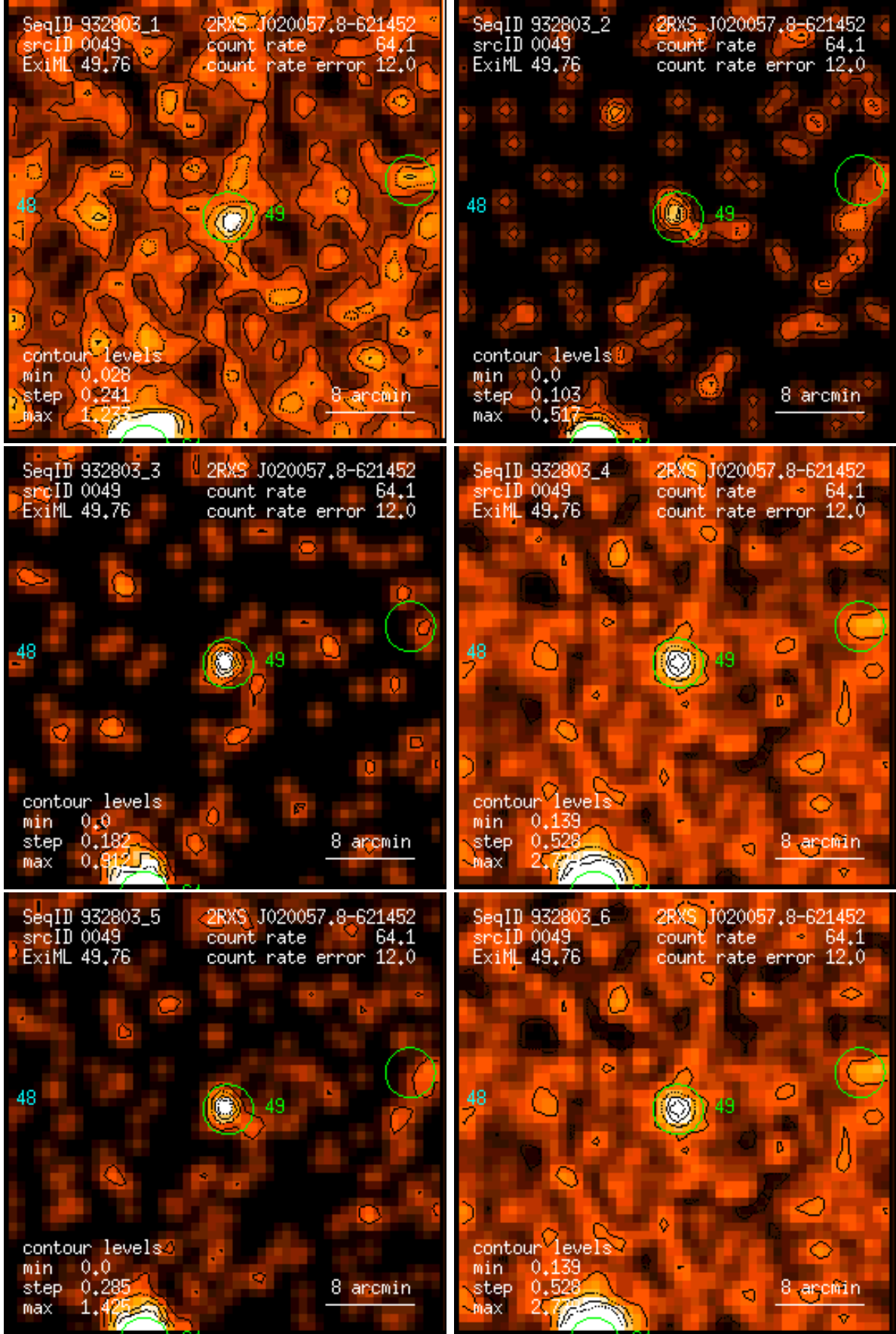
Figure 49: RASS 932803: detection 0049: band rate images, Gaussian filter: (1) PSPC channels 11 – 41, (2) 52 – 90, (3) 91 – 201, (4) 11 – 235, (5) 52 – 201, (6) 11 – 201. Broad band rates in counts/ks. Band rate contour levels in counts/ks/arcmin 2 .
